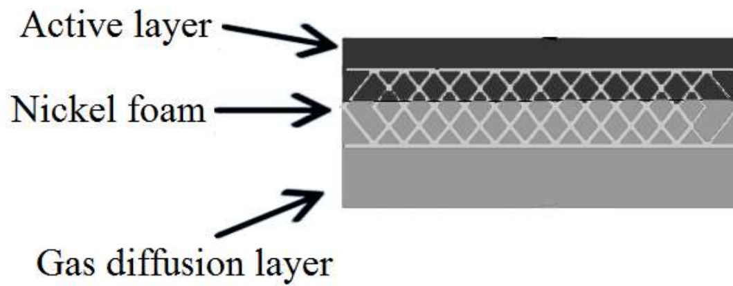
Fig. 8. Schematic diagram of an integrated cathode electrode [121].
