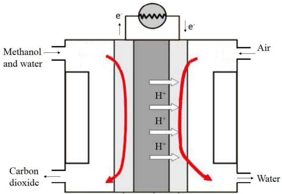
Fig. 3. Schematic diagram of a Direct Methanol Fuel Cell [40].
