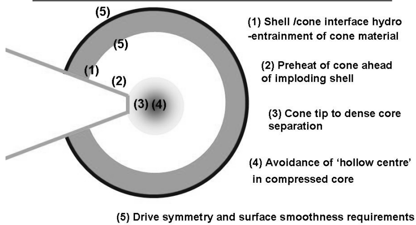
Figure 7: The essential elements and physical constraints of an FI target with cone.
