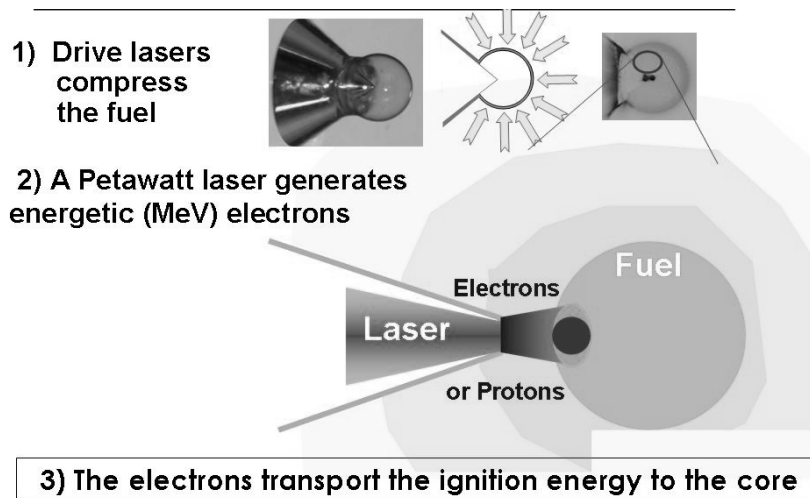
Figure 2 Three essential elements of Fast Ignition
