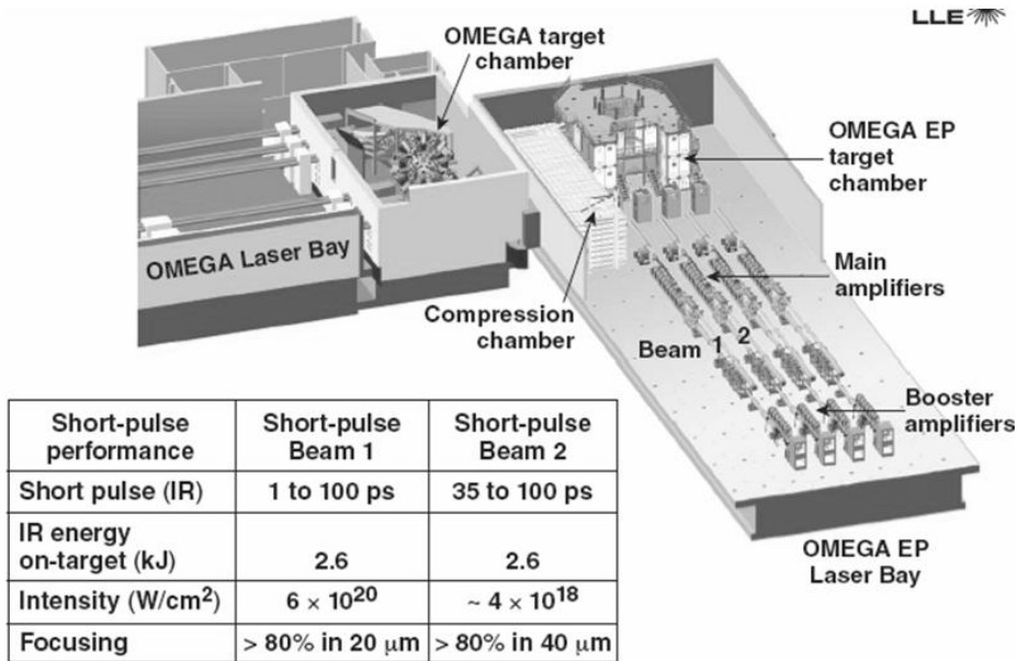
Figure 10: The Omega EP facility to be used for sub-PoP FI experiments
