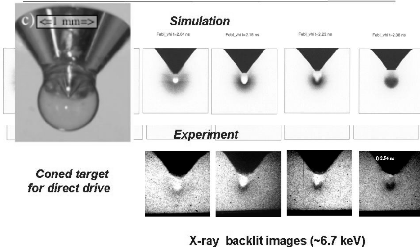
Figure 8: Simulation and experimental results of compression of FI target
