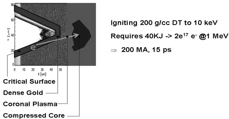
Figure 3 Ignition conditions and fast electron path in an FI target
