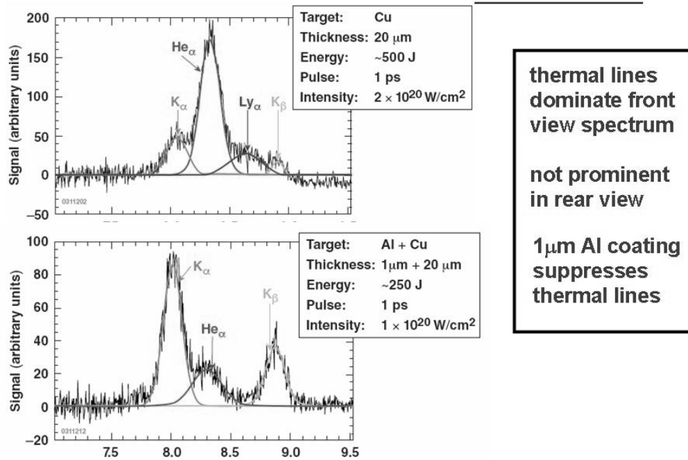
Figure 4: Extreme heating observed in initial layer of slab targets.
