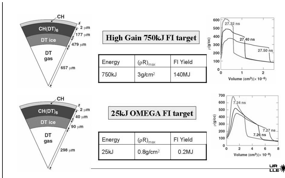
Figure 9 Proposed high gain target for FI.
