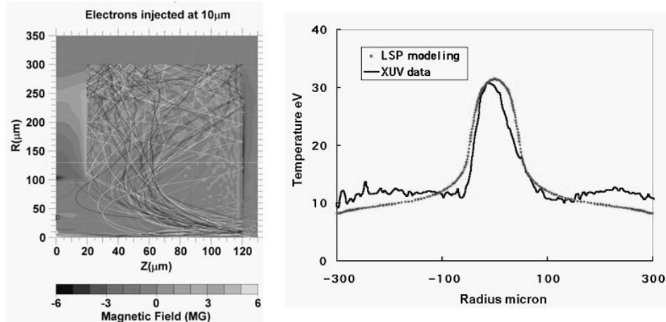
Figure 5: LSP modeling of electron transport and heating on a 100
