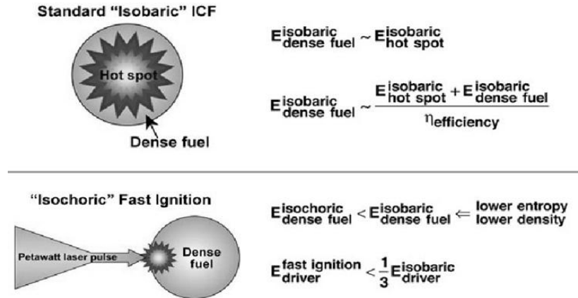
Figure 1: Concept of Fast Fusion
