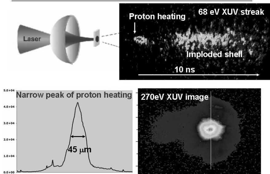
Figure 6: Focusing of protons accelerated from a shaped surface and the resulting heating
