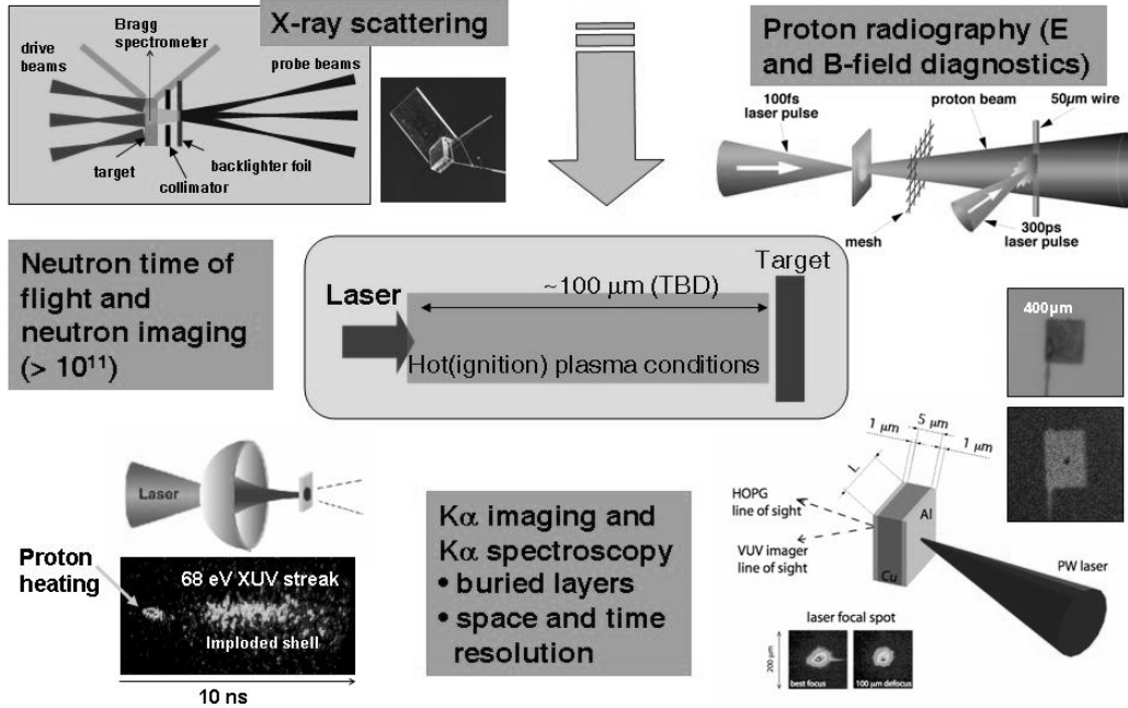
Figure 12: A representation of a partial list of diagnostics to be developed for the sub-PoP experiments.
