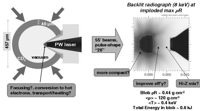
Figure 11: The physical concepts to be examined in preparation for the sub-PoP experiments
