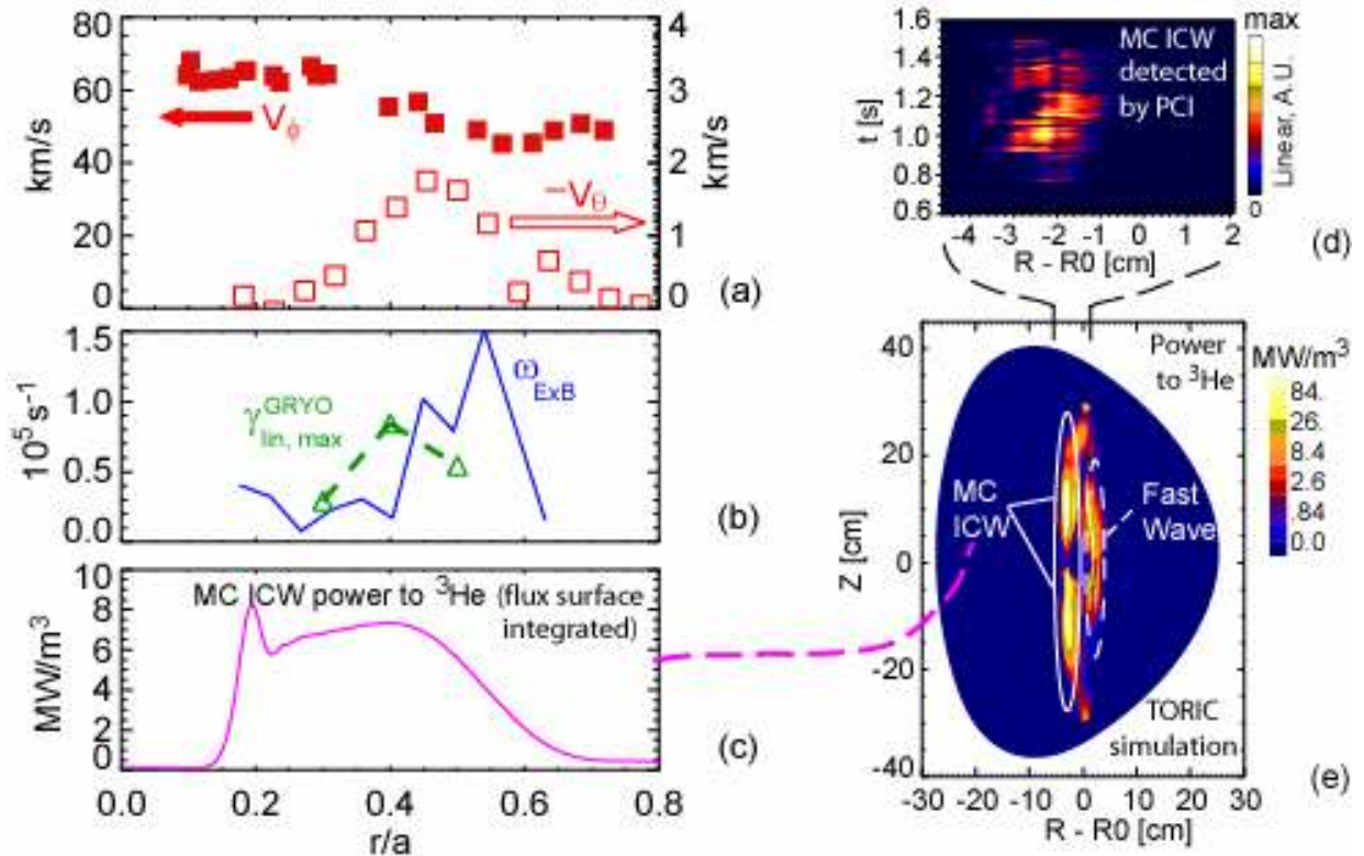
Figure 2: (a) Rotation profiles at t = 1.4 sec of the MC plasma in Fig. ; (b) \omega_{ExB} compared to \gamma_{in,max} from GYRO simulation; (c) Power deposition to ^3\text{He} ions from TORIC; (d) MC ICW in R and t detected by heterodyne PCI; (e) Power deposition in 2-D by TORIC simulation.
