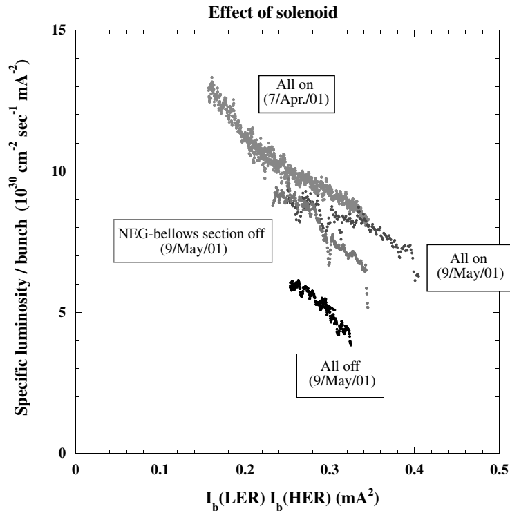
Fig. 4. Luminosity measurements performed in May 2001.
