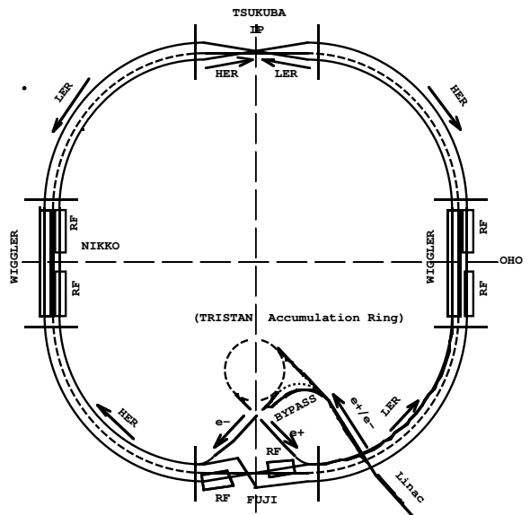
Fig. 2. Schematic of layout of KEKB.
