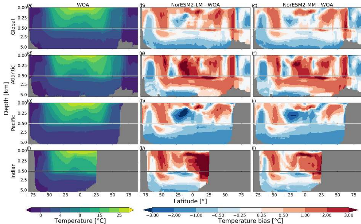
Figure 10. Zonal-mean bias in potential temperature for NorESM2-LM and NorESM2-MM. The bias is taken relative to World Ocean Atlas climatology (Locarnini et al., 2018; Zweng et al., 2018) using the years 1981–2010 in the main ocean basins. Note the change in the vertical scale between the upper 500 m and the lower 4500 m. For the model biases, we show the ensemble-mean bias using three historical members.
