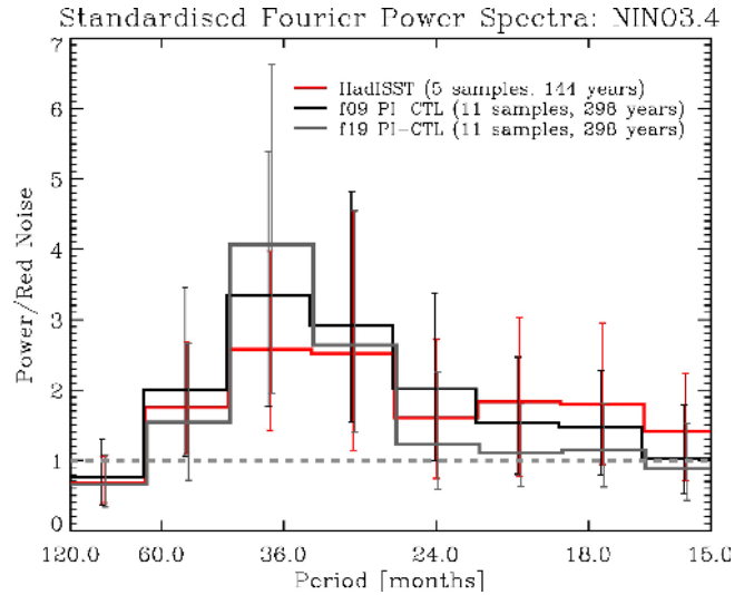
Figure 21. Frequency analysis of El Niño events in NorESM2-MM (f09) and NorESM2-LM (f19) and the Hadley Centre Sea Ice and Sea Surface Temperature dataset (HadISST) v1.1 (Rayner et al., 2003) observed data. Fourier power spectra of NINO3.4 anomalies, normalised to AR1 red-noise model for each (using bootstrapping, 1000 samples).
