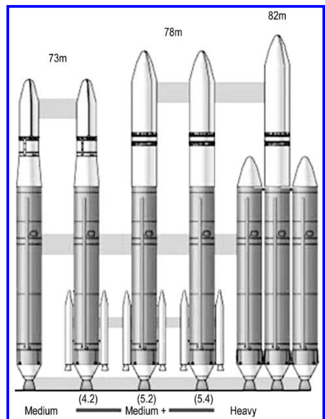
Fig. 8 Delta IV family of launch vehicles.
