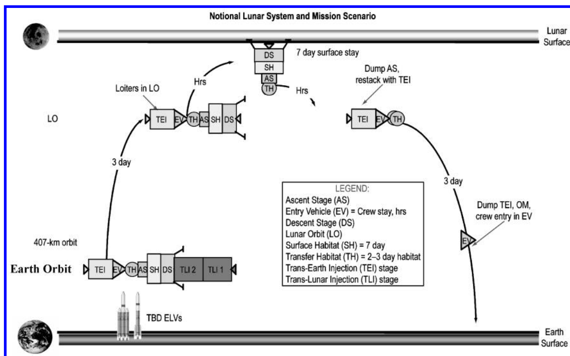
Fig. 13 Notional lunar system and mission scenario.
