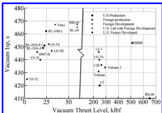
Fig. 3 Existing LO 2 /LH 2 engine production level designs.
