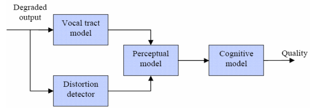
Fig. 8 Non-Intrusive technique
