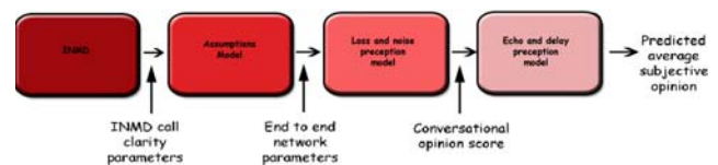
Fig. 9 CCI model
