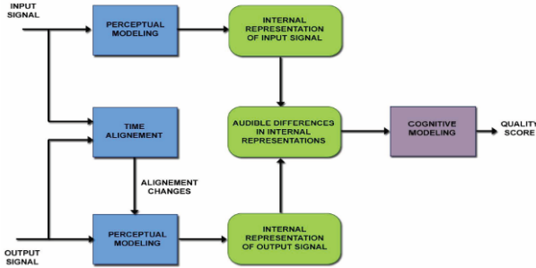
Fig. 7 PESQ model
