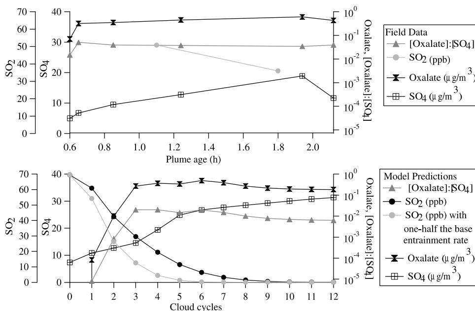
Figure 9. Comparison of flight 5 (9 August 2004) field data and model predictions for \text{SO}_4^{2-} and oxalate growth.
