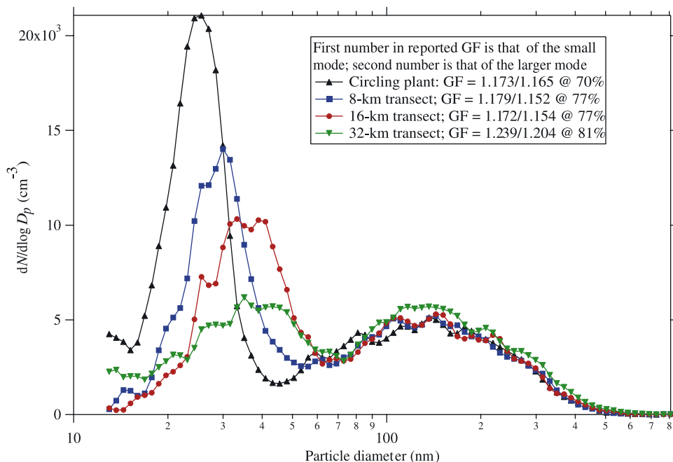
Figure 6. Evolution of the DACAD aerosol size distribution (dry; <20%) for flight 5 on 9 August 2004. GF refers to the aerosol growth factor at the RH value given.
