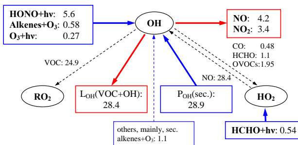
Fig. 5. Average daytime (08:00 h–19:00 h) fluxes of the net radical sources and sinks as calculated by the MCM model. Units are in ppbv h -1 . HONO net contribution (~52%) in this diagram is slightly lower than in the text because [HONO] PSS is calculated here using [OH] calculated by the MCM (~4% higher).
