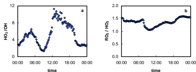
Fig. 6. Average MCM model diurnal variation of (a) HO_2/OH ratio and (b) RO_2/HO_2 ratio.
