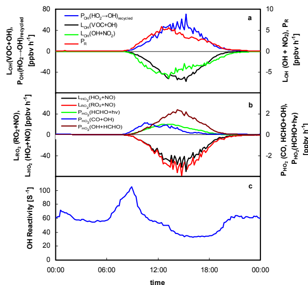
Fig. 4. Production and destruction rates of (a) OH and (b) HO 2 and (c) modelled OH reactivity.
