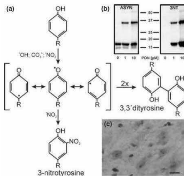
Fig. 7 (a) Mechanism of tyrosine nitration and di tyrosine formation. Tyrosine is oxidized to form an instable tyrosyl radical by various oxidants. In the presence of the ^{\bullet}\text{NO}_2 radical, nitration via a radical based mechanism takes place. Alternatively, when two tyrosyl radicals encounter each other, a covalent di tyrosine bond can be formed. (b) For the western blots, purified alpha synuclein (ASYN) was treated with peroxynitrite as indicated. The membranes were stained with an anti ASYN, or with an anti 3 nitrotyrosine (3 NT) antibody. Peroxynitrite caused nitration of the ASYN monomer. In parallel, a second band with the mass of two ASYN monomers appears. This dimer also exhibited tyrosine nitration. (c) Nitrated ASYN is observed in the aging brain (McCormack et al. 2012), Parkinson's disease (PD) (Giasson et al. 2000), or during experimental neurodegeneration (McCormack et al. 2008). As an example, dopaminergic neurons in the substantia nigra of a squirrel monkey, treated with MPTP, are shown. Widespread immunoreactivity (brown) for nitrated ASYN is detected. The darker dots within neurons represent neuromelanin. The tissue was obtained from an animal four weeks after a single subcutaneous injection of 1.75 mg/kg MPTP. Scale bar 10 \mu\text{m} .
