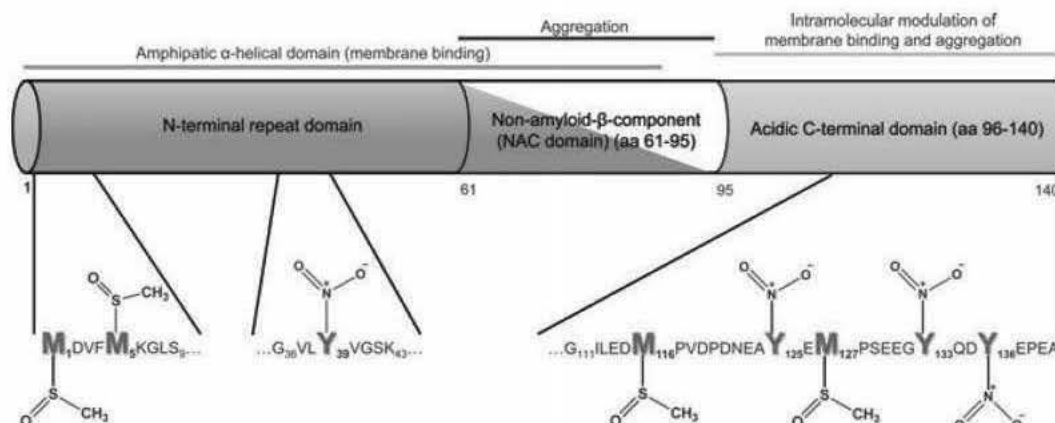
Fig. 4 Oxidative modifications of alpha synuclein (ASYN). The 140 amino acid protein is composed of an N terminal domain that adopts an \alpha helical conformation when in contact to a water lipid interphase. The central non amyloid component (NAC) region is mainly involved in the aggregation of the protein, while the acidic C terminal region has
