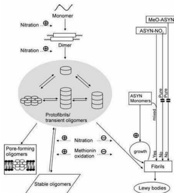
Fig. 5 Regulation of alpha synuclein (ASYN) aggregation by oxidative modifications. Treatment with peroxynitrite or other oxidants accelerates the formation of covalently linked dimers and/or stable oligomers that no longer contribute to fibrillation. In contrast, unstable oligomers, originating from unmodified ASYN, represent an inhomogenous mixture of spherical, chain like, or annular protofibrils. Some of these transient structures, for example, can form membrane pores and hence are considered cytotoxic. Nitrated monomeric ASYN alone does not contribute to fibrillation under conditions that favor fibril formation by non modified ASYN. The situation is different when nitrated ASYN is added to non modified ASYN. In this case, the modified monomers serve as aggregation seed (right) and accelerate fibrillation.
