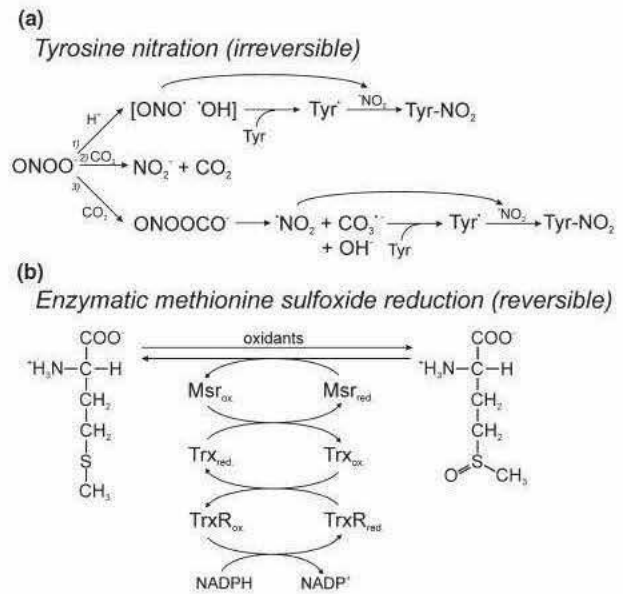
Fig. 6 Chemical biology of tyrosine nitration and methionine sulfoxide reduction. (a) Tyrosine nitration is an irreversible reaction. At cellular pH, most peroxynitrite is present in its deprotonated form, but peroxynitrous acid (ONOOH) is formed rapidly by protonation ( \text{pK}_a 6.6). It is chemically unstable and undergoes homolysis into the \cdot\text{NO}_2 radical and the hydroxyl radical ( \cdot\text{OH} ). The \cdot\text{OH} or the \cdot\text{NO}_2 radical can react with tyrosine residues to form tyrosyl radicals. In the presence of large amounts of bicarbonate, peroxynitrite can also react with \text{CO}_2 . Two thirds of the resultant reaction product decomposes to yield nitrite ( \text{NO}_2^- ) and \text{CO}_2 (2), while about one third generates the \cdot\text{NO}_2 radical and \text{CO}_3^{\cdot-} (3). The \cdot\text{NO}_2 from (1) and (3) can react with the tyrosyl radical to form 3 nitrotyrosine (3 NT). (b) Methionine oxidation is a biologically reversible reaction. The reduction of methionine sulfoxide is catalyzed by methionine sulfoxide reductase (Msr). This enzyme uses the thioredoxin reductase (TrxR) thioredoxin (Trx) system, driven by NADPH for its enzymatic oxidation reduction cycle.
