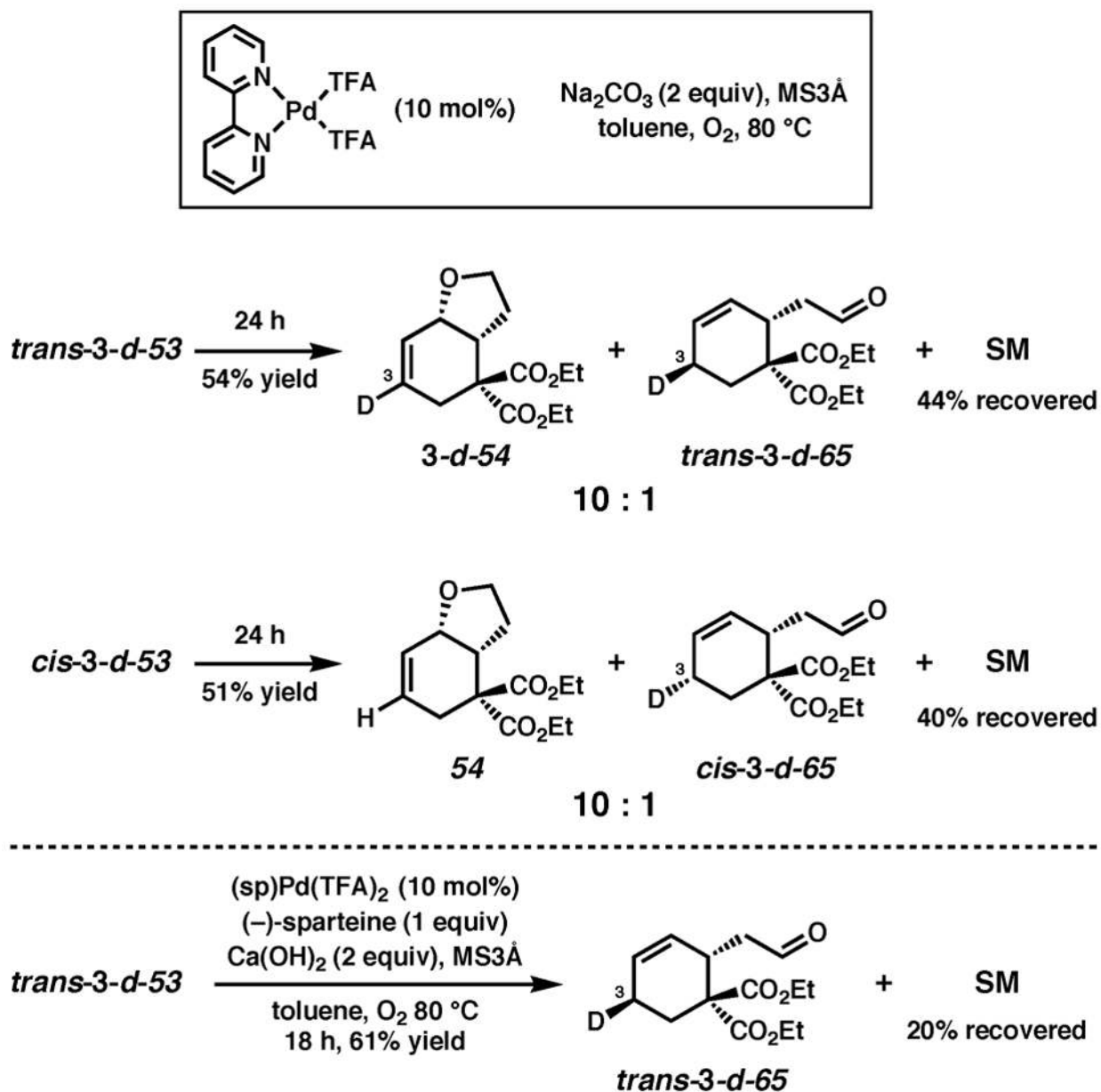
Scheme 4. Cyclization of deuterium-labeled primary alcohol substrates with dipyrindyl as ligand.
