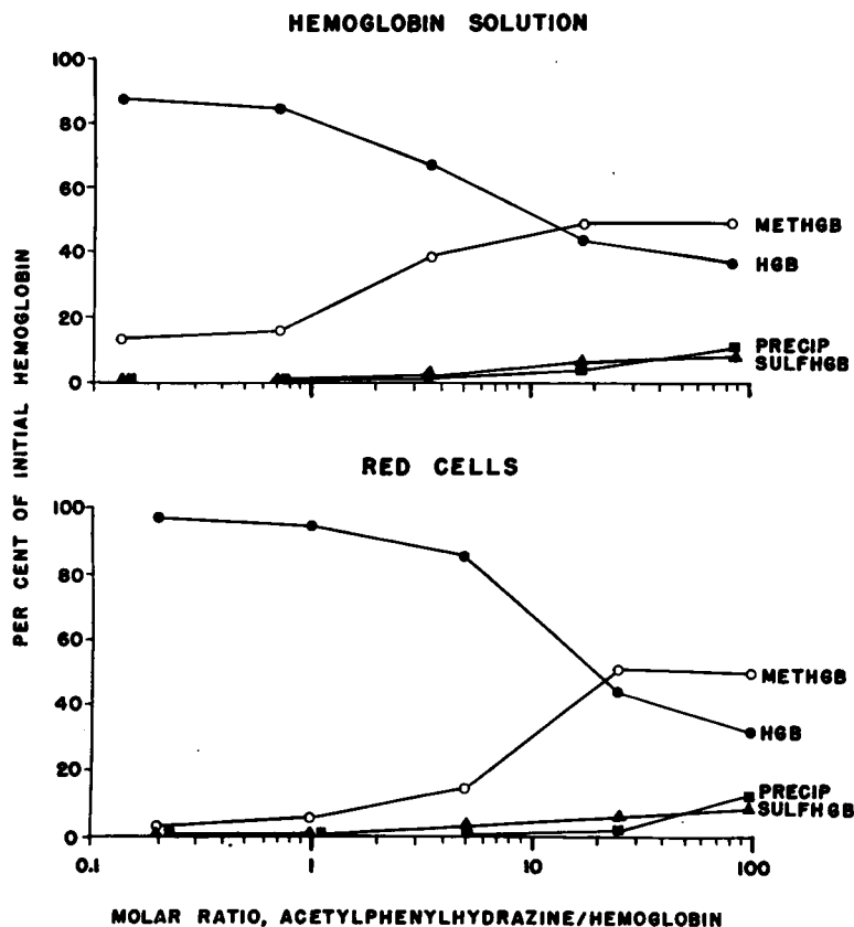
FIG. 2. EFFECTS OF VARIOUS QUANTITIES OF ACETYPHENYLHYDRAZINE ON HEMOGLOBIN IN SOLUTION (ABOVE) AND WITHIN WASHED RED CELLS (BELOW). Apart from the fact that the solutions of crystalline hemoglobin contained 12 per cent methemoglobin to begin with, the levels of methemoglobin (empty circles), sulfhemoglobin (black triangles), and of hemoglobin (ferrohemoglobin) (black circles) were similar in the two preparations. In the red cell preparation the water-soluble precipitate value (black squares) was corrected for the weight of the stroma of untreated cells.
