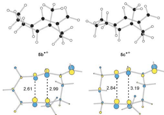
Figure 6. Structures and singly occupied MOs of 1-methyl-8-methylene-1,6-cyclodecadiene radical cations 5b^+ and 5c^+ . Numbers indicate distances in Å.
