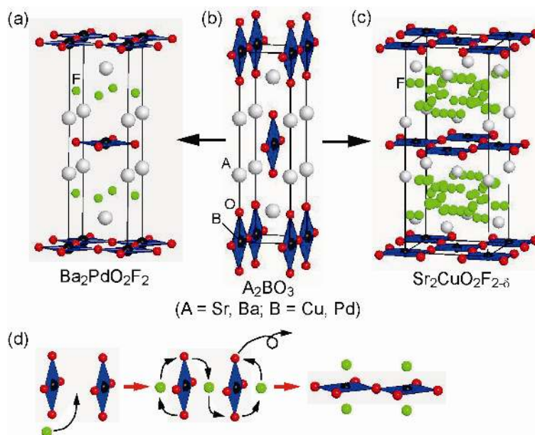
Figure 8. (a), (b), (c) Fluorination of A_2BO_3 to A_2BO_2F_{2-\delta} ( A = \text{Sr}, \text{Ba}; B = \text{Cu}, \text{Pd} ). (d) Rearrangement of oxide and fluoride anions during fluorination reaction.
