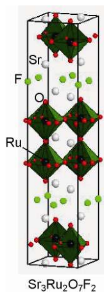
Figure 7. Crystal structure of \text{Sr}_3\text{Ru}_2\text{O}_7\text{F}_2 .
