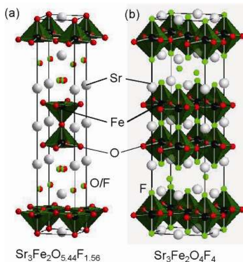
Figure 10. Crystal structure of (a) \text{Sr}_3\text{Fe}_2\text{O}_{5.44}\text{F}_{1.56} , and (b) \text{Sr}_3\text{Fe}_2\text{O}_4\text{F}_4 .
