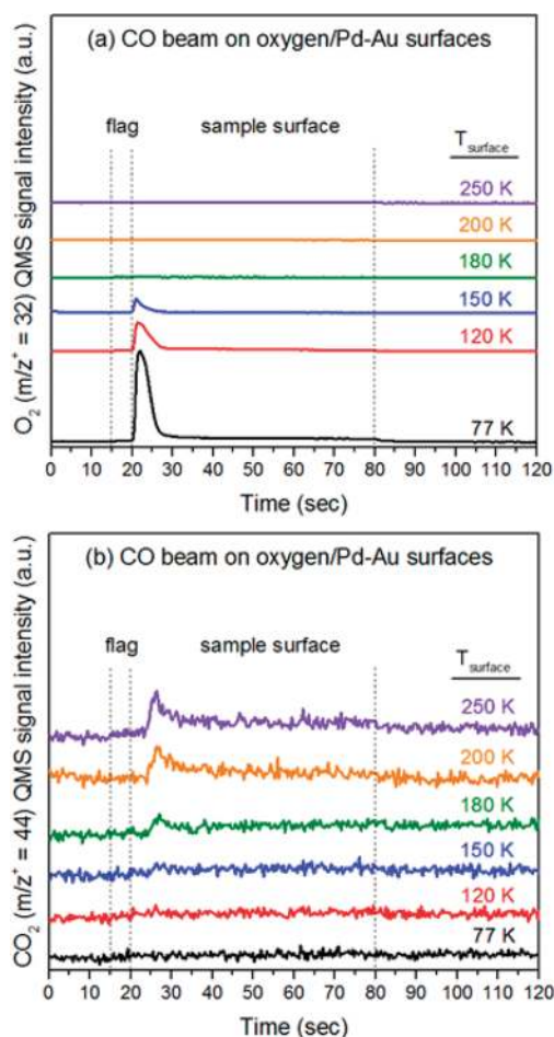
Figure 6. (a) O_2 ( m/z^+ = 32 ) and (b) CO_2 ( m/z^+ = 44 ) QMS signals during CO-RMBS on the oxygen-pre-saturated Pd/Au(111) bimetallic surface at various surface temperatures.
