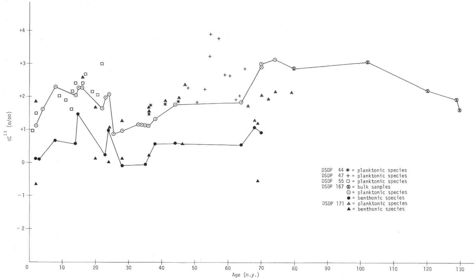
Figure 8. Carbon isotope results from Sites 47, 55, 167, and 171 plotted as a function of sample age.
