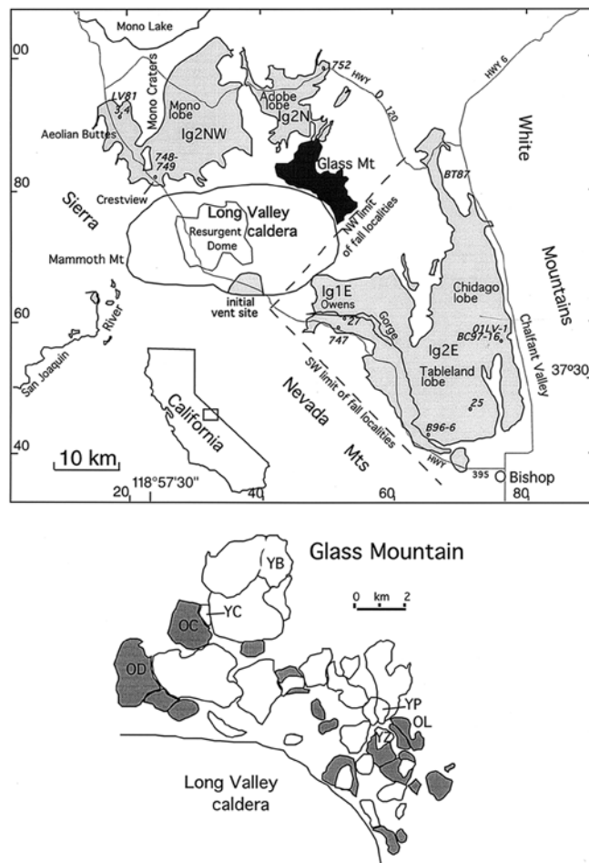
Fig. 1. Map of Long Valley Caldera and vicinity ( top ) and enlargement of Glass Mountain area ( bottom ). Lobe names are from Hildreth (1979), new names of ignimbrite and fall units (Ig, F, Table 1) are from Wilson and Hildreth (1997); sample localities and abbreviated numbers (99LV-) are shown for Bishop Tuff and analyses are given in Table 1. Numbers 20, 40, 60, 80 next to tic marks on the frame are UTM coordinates. At Glass Mountain, Older (2.1–1.2 Ma) domes are dark , Younger (1.2–0.79 Ma) domes are white . Long Valley caldera is surrounded by Paleozoic and Mesozoic Sierra Nevada granitoids, and is superimposed on the major Sierran fault (Bailey 1989). Many of these country rocks are present as clastic inclusions throughout the BT and were used to infer the sequence of caldera ring fracture propagation during the 0.76-Ma caldera-forming eruption (Hildreth and Mahood 1986; Wilson and Hildreth 1997). Sierra Nevada granitoids in the vicinity of Long Valley have \delta^{18}\text{O}(\text{WR}) values of +8 to +9‰ (Masi et al. 1981); metasedimentary rocks range from +8 to +29‰ in some metacarbonates of Mt. Morrison roof pendant (Smith and Suemnicht 1991; Lackey and Valley 1999) to 2‰ in hydrothermally altered volcanic rocks below BT exposed at depths down to 2 km in drill holes (McConnell et al. 1997). Plutonic and metasedimentary rocks also show a wide range in Sr isotope compositions (0.706–0.725), usually exceeding that of BT (Goff et al. 1991)
