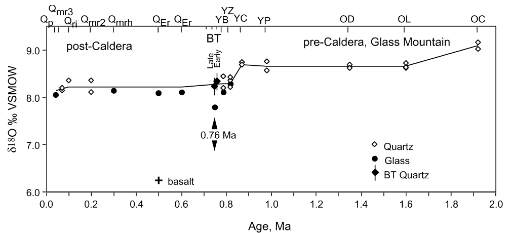
Fig. 2. Evolution of \delta^{18}\text{O} values in Glass Mountain-Bishop Tuff magma system. Unit names are from Table 1. Notice larger range and slightly higher \delta^{18}\text{O} (quartz) values in older Glass Mountain lavas, similar \delta^{18}\text{O} values of 2 youngest Glass Mountain lavas and Bishop Tuff, and an overall similarity of \delta^{18}\text{O} values in post-caldera lavas. Solid line represents the trend for melt in equilibrium with quartz (see text)
