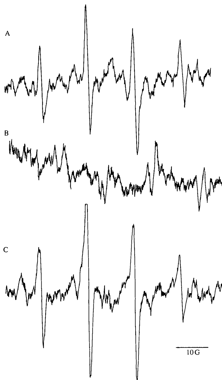
Fig. 4. Electron paramagnetic resonance spectra from tissue suspensions of naturally occurring apozooxanthellate specimens of Anthopleura elegantissima . Despite the absence of zooxanthellae, DMPO/ \cdot OH signals are detected when apozooxanthellate anemones are illuminated (A), compared to unilluminated sample (B). This radical production is clearly not dependent on photosynthetically induced hyperoxia and, as expected, DCMU has no effect (C). The larger peaks and increased baseline noise compared with other figures are due to increased receiver gain ( 8 \times 10^4 ), whereas larger peak heights in C compared with A probably result from there being more biomass in the flat cell. Spectrometer settings as in Fig. 3, except 8 min scan.
