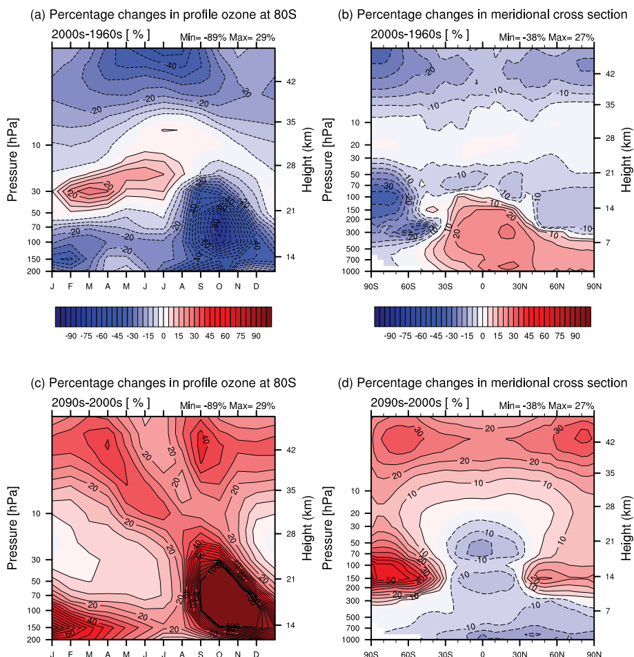
Fig. 13. (a) Annual cycle at 80^{\circ} S and (b) meridional cross-section of the percentage differences in ozone between the 1960s and the 2000s. (c, d) Same as (a, b), but for the differences between the 2000s and the 2090s. The future GHG scenario shown is RCP 4.5 in the troposphere and SRES A1B in the stratosphere.
