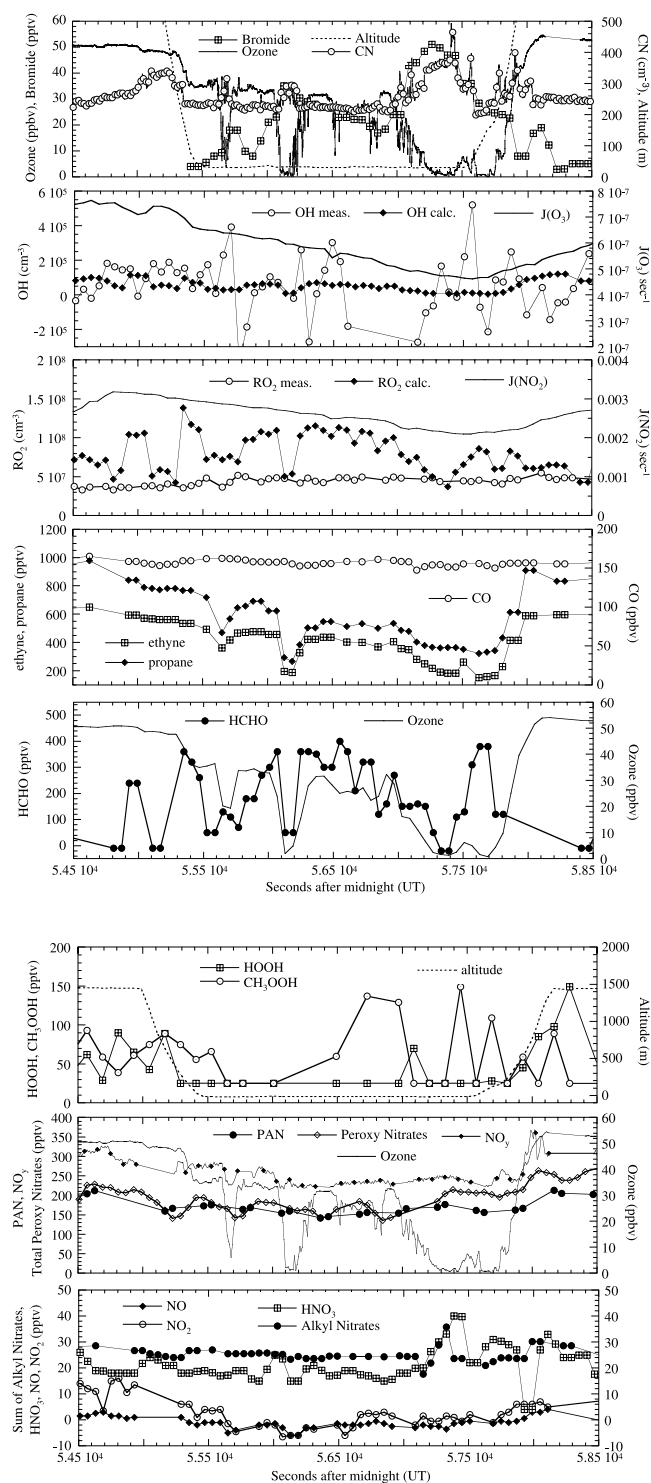
Figure 8. (a) Other constituent measurements for the low altitude leg over the Arctic Ocean for the 23 March flight. Bromide is soluble bromide measured by the mist chamber instrument and the detection limit is \sim 2 pptv. Soluble bromide was usually only measured when at low altitude. The data are from a 1 min average merged data file except for the top panel where ozone and CN are 1 s values. (b) As in Figure 8a. The ozone and NO y data in the middle panel are at 10 s resolution. All other data are from the 1 min merged file. The detection limit of the HOOH and CH 3 OOH instruments is \sim 25 pptv.
