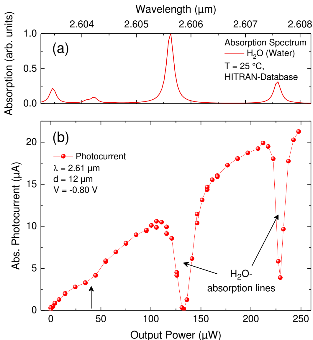
Figure 5: (a) Water absorption spectrum at T = 25\text{ °C} at around 2.61\text{ }\mu\text{m} . The data is taken from the HITRAN database. [64] (b) Absolute photocurrent as a function of the laser output power incident on the optical aperture of the Au-ring shaped contact. The output power is tuned via the diode current. Due to Joule heating, the emission wavelength undergoes a red-shift with increasing output power. When the emission wavelength crosses a water absorption line, a drop in the photocurrent is observed. These local minima are indicated by black arrows.
