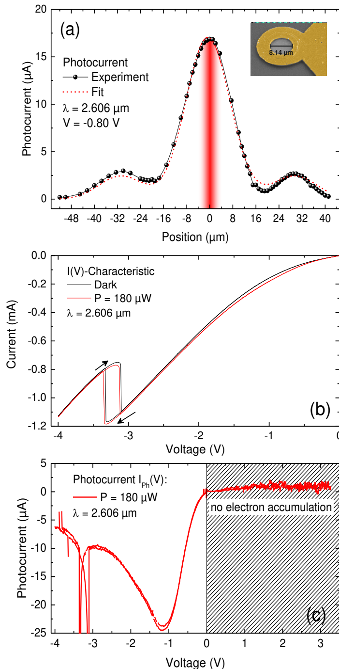
Figure 4. Mid-infrared photoresponse at room temperature for illumination with a mono-mode diode laser of the wavelength \lambda = 2.606 \mu\text{m} . (a) Cross-section of the laser intensity profile given by the photocurrent (black spheres) as a function of diode position. The inset shows a colored SEM image of an RTD mesa structure with diameter of nominally d = 12 \mu\text{m} and Au-ring shaped contact. The optically accessible area has a diameter of d = 8.14 \mu\text{m} . From the best fit function (red dashed line) of the convolution, the fraction of light power incident on the RTD is calculated to be about 5.8%. (b) I(V) -characteristics in the dark (black) and under illumination with \lambda = 2.606 \mu\text{m} and P \approx 180 \mu\text{W} . The bistability is due to a series resistance of R = 1.0 \text{ k}\Omega . (c) Photocurrent-voltage characteristics I_{\text{ph}}(V) for an incident light power of P \approx 180 \mu\text{W} . Only for negative bias voltages, photogenerated electrons can accumulate in the vicinity of the RTS and modulate the tunneling current via Coulomb interaction.
