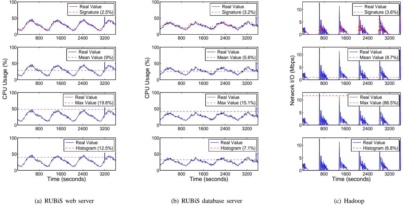
Fig. 7. Resource usage traces and prediction comparison for RUBiS and Hadoop. The mean prediction errors are shown in the legend.
