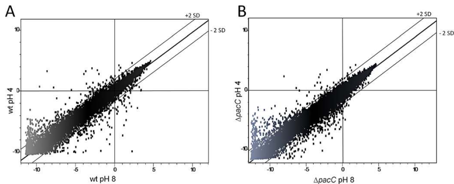
Figure 4 Scatter plot representation of microarray data from wt (A) and ΔpacC (B) at pH 8 compared to pH 4. Each dot represents the microarray signal of the particular gene. The best-fit linear trend and the \pm 2 standard deviation (SD) lines (dashed) are indicated.
