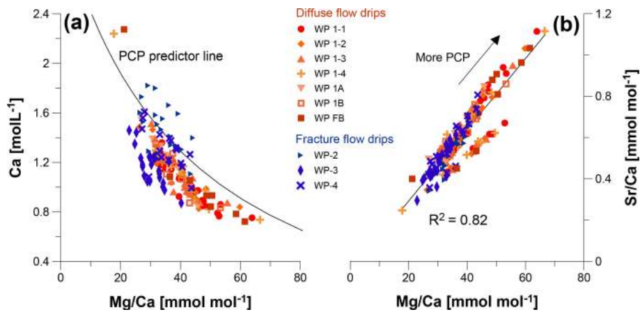
Figure 10. Waipuna Cave drip waters sampled during the monitoring period October 2016 to January 2019. (a) Ca concentration versus Mg/Ca ratios. (b) Mg/Ca versus Sr/Ca; R^2 = 0.82 , p < 0.001 . The orange symbols correspond to diffuse flow drip sites and blue symbols signify fracture flow drip sites. The two different trends evident in the relationship between Mg/Ca and Sr/Ca will be discussed in Sect. 5.5.
