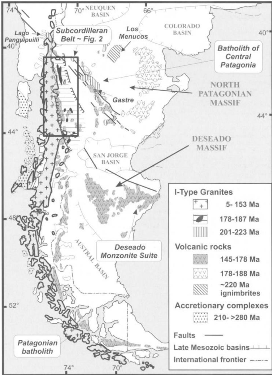
Fig. 1. Distribution of Triassic and Jurassic magmatism and location of the main sedimentary basins in Patagonia (modified from Rapela 2001). The boundary of the Subcordilleran belt (cross-hatched area inside the box) is after the palaeogeographical reconstruction of the Liassic basin by Lizaín (1999), while the main areas of the Triassic–Early Jurassic accretionary prism in the Pacific margin are from Thomson & Hervé (2002). Isotopic ages for the Chon Aike Province are from Pankhurst et al. (2000): rocks of V 1 (c. 188–178 Ma) occur in the eastern North Patagonian Massif; those of V 2 (c. 172–162 Ma) and V 3 (c. 157–153 Ma and younger) are not distinguished. See text for data sources and discussion of the isotopic ages of the I-type granites: the coastal batholith (and the sedimentary basins outlined) are largely post-break-up.
