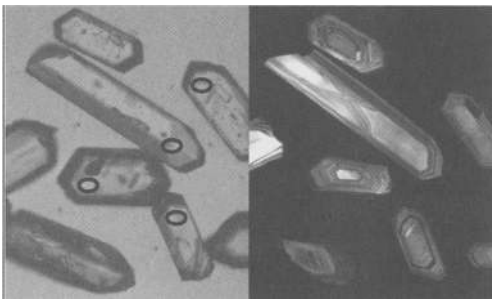
Fig. 4. Reflected light and cathodo-luminescence images of analysed zircon grains from sample SER-046 (La Angostura granite). The large grain is c. 250 \mu\text{m} in length. SHRIMP ablation spots are marked on the left-hand image, chosen to avoid cracks and inclusions.
