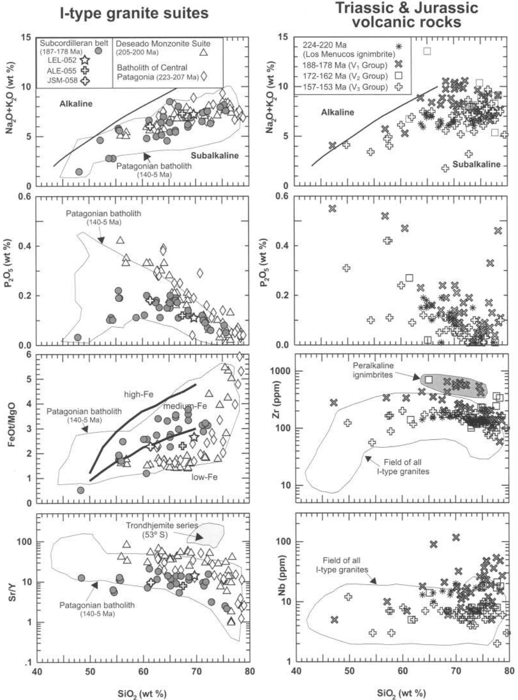
Fig. 6. Harker plots for Triassic–Jurassic I-type granites and volcanic rocks from Patagonia. The line dividing alkaline and subalkaline fields is from Irvine & Baragar (1971) while the fields for high, medium and low Fe are after Arculus (2003). Data sources for the Triassic and Jurassic volcanic rocks: Pankhurst & Rapela (1995); Rapela (2001) and unpublished data from a British Antarctic Survey–Argentine joint expedition (P. T. Leat, pers. comm. 2003). Data sources for the I-type granites are the same as reported in Figure 3.
