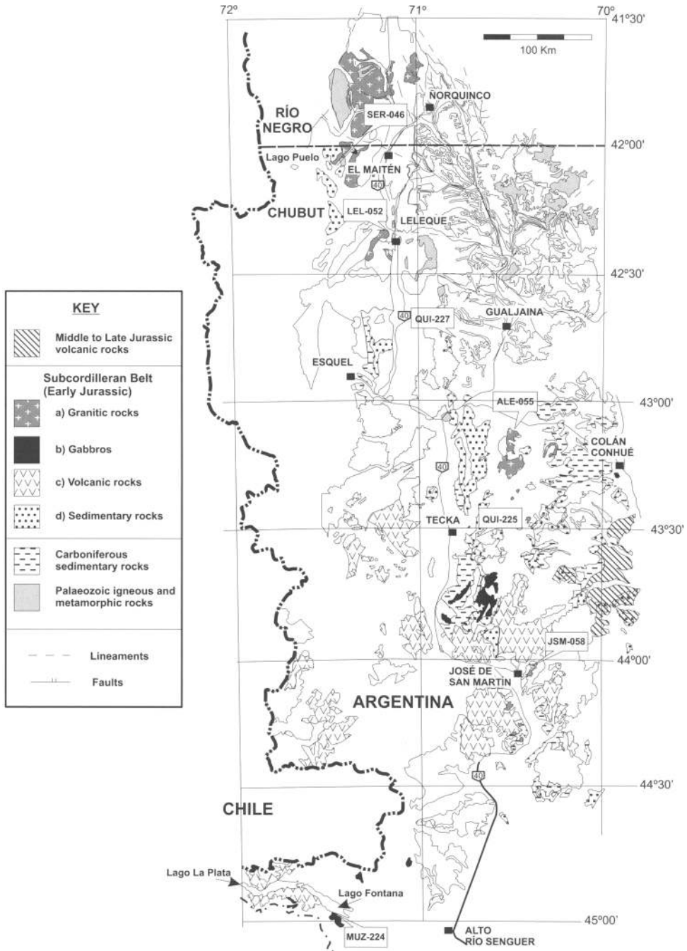
Fig. 2. Simplified geological map of the Subcordilleran sector between 41°30' and 44°15' S.
