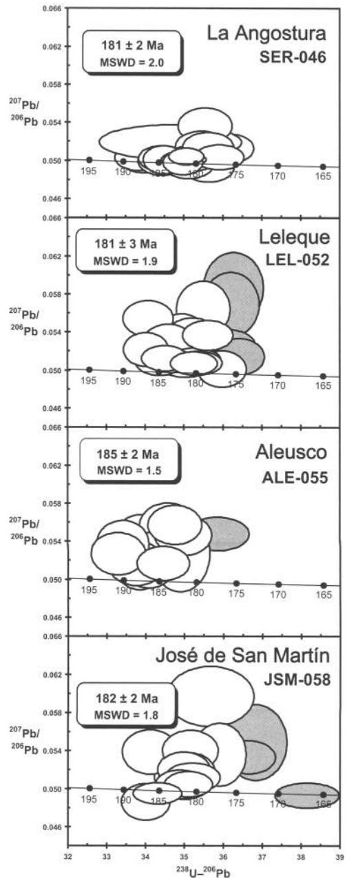
Fig. 5. Tera–Wasserburg plots of SHRIMP zircon data for magmatic units of the Subcordilleran plutonism of northwestern Patagonia. Open ellipses are 68% confidence limits for analyses of crystal tips, uncorrected for common Pb. Age errors are reported at 95% confidence limit. Shaded ellipses are for data outside the acceptable range for definition of a single event, probably due to radiogenic Pb-loss; these were excluded from the calculation of crystallization ages. MSWD, Mean Square of Weighted Deviates.
