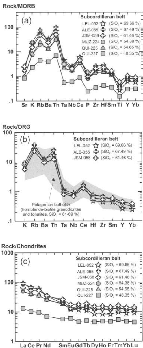
Fig. 7. (a) Trace element abundances in granitic and basic rocks of the Subcordilleran belt normalized to MORB (Pearce 1983). (b) Trace element abundances in granitic rocks of the Subcordilleran belt normalized to ocean ridge granite (ORG, Pearce et al. 1984). The field of the Patagonian batholith has been constructed from chemical data for hornblende–biotite granodiorites and tonalites (61–69% SiO 2 ) reported by Ghiara et al. (1997), Pankhurst et al. (1999) and unpublished data of C. W. Rapela at 41° S. (c) Chondrite-normalized REE patterns of representative samples from the Subcordilleran plutonic belt.
