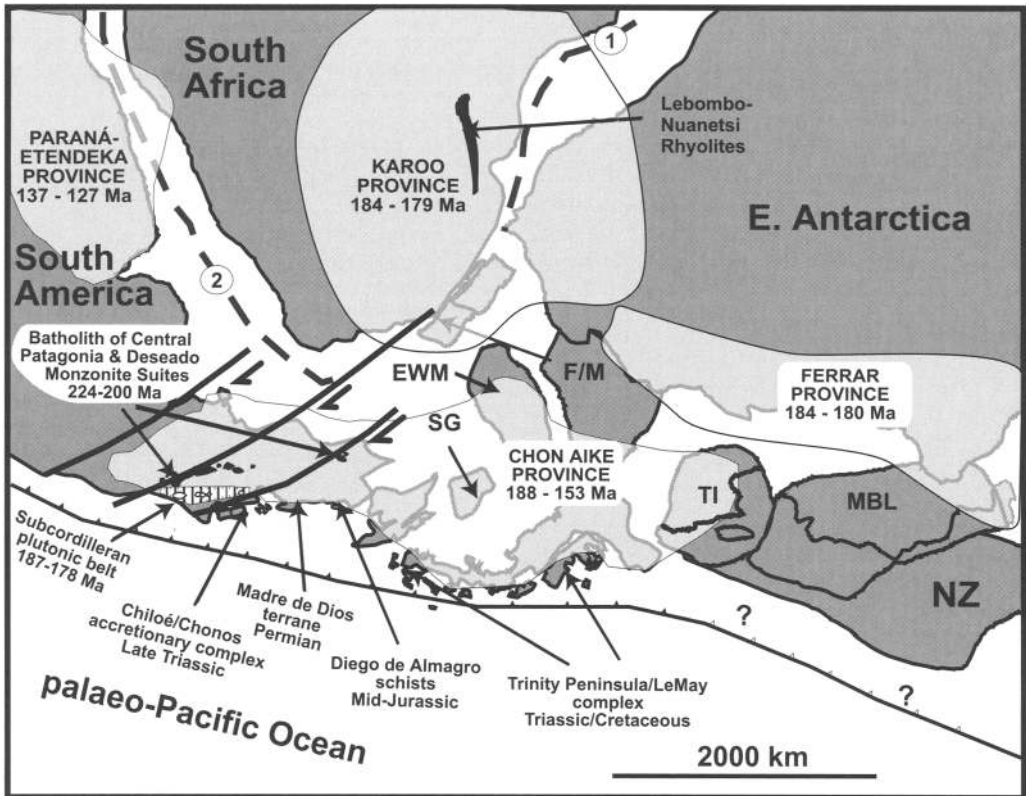
Fig. 10. Schematic Early Jurassic palaeogeographical reconstruction of southwestern Gondwana (modified after the Early Jurassic base map of Storey et al. 1992). A tight fit is obtained by a palinspastic restoration of southern South America and the Antarctic Peninsula as proposed by MacDonald et al. (1998), involving 50% closing of the largest southernmost Mesozoic basins (Austral, San Jorge and Colorado, Fig. 1), reducing by 20% the size of the Antarctic Peninsula to remove approximately Late Mesozoic and Tertiary crustal growth, and allowing for moderate dextral displacement of about 140 km of large crustal blocks along major fault systems bounding the North Patagonian and the Deseado massifs. Partial restoration of the Cretaceous–Cenozoic oroclinal curvature in the southern tip of South America and the Antarctic Peninsula has also been performed (e.g. Kraemer 2003). Triassic and Early Jurassic accretionary prism after Thomson & Hervé (2002). Location and timing of the Jurassic magmatic provinces are after Pankhurst et al. (2000), while heavy broken lines that show the sites of the initial areas of the Indian Ocean (1) and the future South Atlantic Ocean (2) are from Cox (1992). Crustal blocks: EWM, Ellsworth–Whitmore mountains; SG, South Georgia; F/M, Falkland/Malvinas microplate; TI, Thurston Island; MBL, Marie Byrd Land; NZ, New Zealand.
