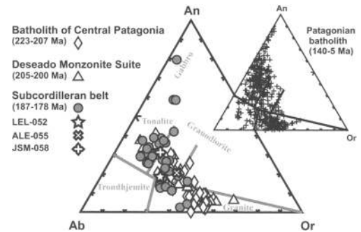
Fig. 3. Normative Ab–An–Or diagram for the Mesozoic and Cenozoic I-type granites of Patagonia. Data for the Subcordilleran belt are from Gordon & Ort (1993), Busteros et al. (1993), Haller et al. (1999) and this paper; for the Deseado Monzonite Suite from Rapela et al. (1996); and for the Batholith of Central Patagonia from Rapela et al. (1992). The normative composition of the Patagonian batholith is based on 415 chemical analyses reported for different latitudes of the body: 53^{\circ} S (Bruce 1988), 48^{\circ} S (Weaver 1988), 45 – 46^{\circ} S (Wells 1978), 44 – 46^{\circ} S (Pankhurst et al. 1999), 43^{\circ} S (Haller 1985), 42^{\circ} (Ghiara et al. 1997) and 40 – 41^{\circ} S (Rapela unpublished data).
