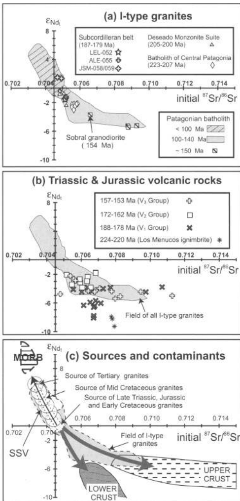
Fig. 8. Variation of \epsilon_{Nd_t} versus initial ^{87}Sr/^{86}Sr for the Late Triassic and Jurassic magmatic units of Patagonia. Data sources for I-type granites: Rapela et al. (1992), Rapela & Pankhurst (1996), Pankhurst et al. (1999) and Pankhurst & Hervé, unpublished data. For volcanic rocks: Pankhurst & Rapela (1995) and Pankhurst, unpublished data. The fields for the upper and lower crust in (c) are from the Chilean accretionary prism and the North Patagonian Massif V_1 rhyolite group, respectively (Pankhurst et al. 1999). The MORB (mid-ocean ridge basalts) field is from Zindler & Hart (1986), while SVZ (mafic Southern Volcanic Zone) is from Gorring & Kay (2001 and references therein).
