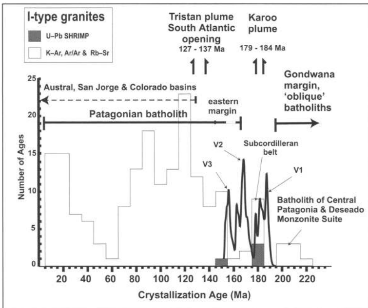
Fig. 9. Histograms of ages for the Mesozoic and Cenozoic I-type granites of Patagonia. Data sources: Patagonian batholith between 45° and 53° S (Bruce et al. 1991; Pankhurst et al. 1999; Suarez & De la Cruz 2001); Subcordilleran belt (Lizuaín 1981; Gordon & Ort 1993; Haller et al. 1999; this paper); Deseado Monzonite Suite (Pankhurst et al. 1993); Batholith of Central Patagonia (Rapela et al. 1992). Cumulative probability curve and age groups for the Jurassic rhyolite province of Patagonia are from Pankhurst et al. (2000). Inferred ages for the Karoo and Tristan mantle plumes are from Duncan et al. (1997) and Turner et al. (1994), respectively.
