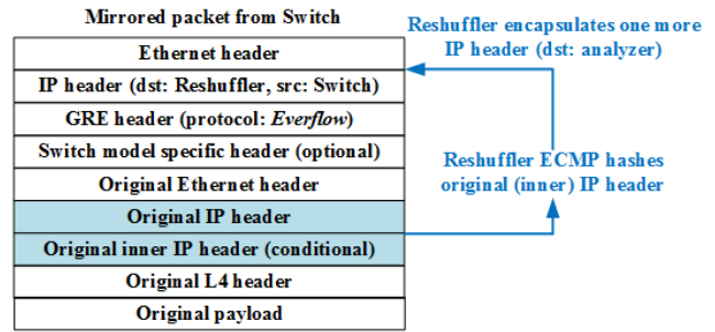
Figure 6: Format of mirrored packet
