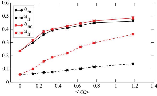
FIG. 17. (Color online) Normal and tangential force anisotropies a_n and a_t , and radial and orthoradial force anisotropies a'_{fn} and a'_{ft} , as a function of \langle\alpha\rangle in the residual state. The error bars represent the standard deviation in the residual state.
