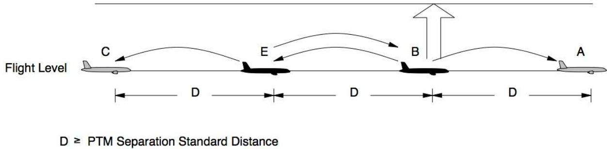
Figure A9-1. Aircraft leaving a chain vertically with a chain remaining
