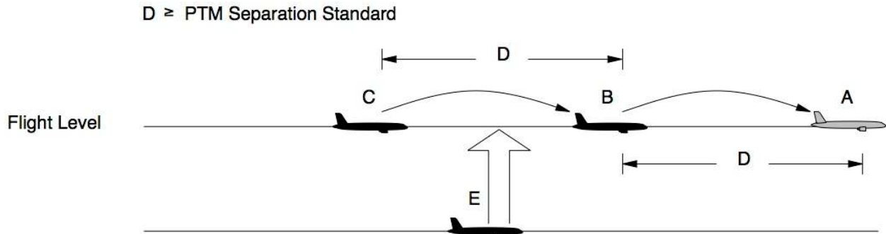
Figure A6-3. Joining a string by climbing or descending to the PTM string flight level, between the aircraft
