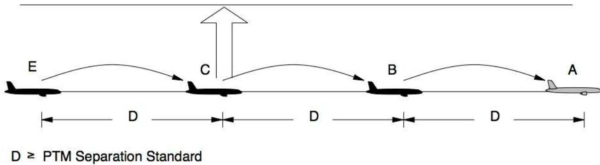
Figure A8-3. Departing a string by climbing or descending, inside the string
