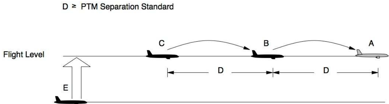
Figure A6-1. Joining a string by climbing or descending to the PTM string flight level, trailing
