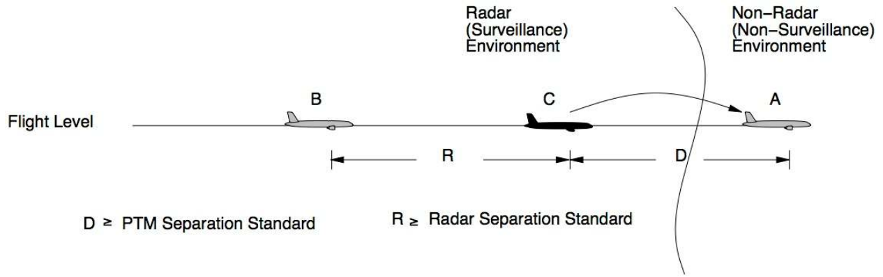
Figure A4-5. Formation of string horizontally, transition from radar to non-radar environment
