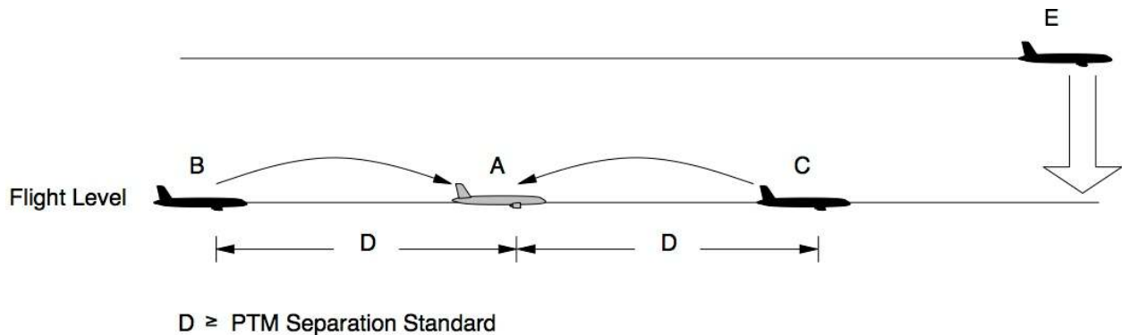
Figure A6-2. Joining a string by climbing or descending to the PTM string flight level, leading
