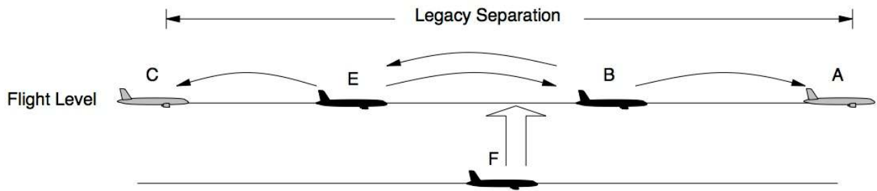
Figure A7-1. Joining a chain by climbing or descending to the chain flight level
