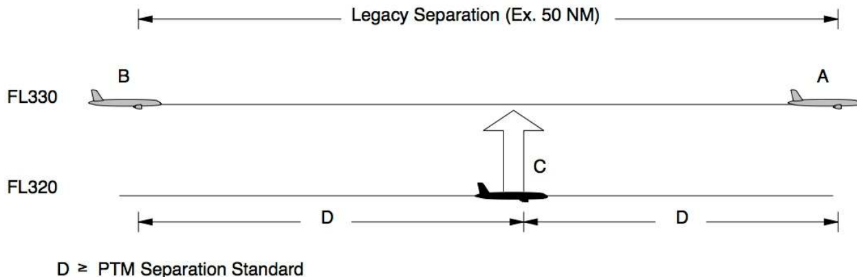
Figure A5-1. Formation of chain by climbing or descending between designated aircraft
