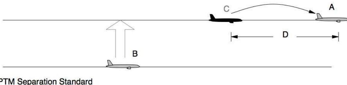
Figure A5-2. Designated aircraft climbs or descends to the flight level of the PTM pair
