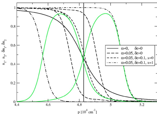
FIG. 5. (Color online) The dependence of the occupation probabilities of two hyperfine states on the momentum. The Fermi momentum k_F=4.83 \times 10^4 \text{ cm}^{-1} is indicated by the vertical line. The labeling of the lines is as follows: \alpha=0, \delta\epsilon=0 (solid line), \alpha=0.05 and \delta\epsilon=0 (long-dashed lines), \alpha=0.05, \delta\epsilon=0.1 , and x=0 (short-dashed lines), and x=1 (dash-dotted lines). The bell-shaped light curves show the anisotropy—the difference between the x=1 and x=0 occupation numbers—for \alpha=0.05, \delta\epsilon=0.1 . The remaining parameters are as in Fig. 1.
