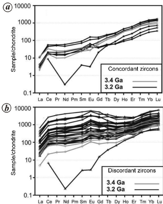
Figure 4. Chondrite-normalized REE patterns for (a) concordant; and (b) discordant zircons from quartzite of Girar supracrustal belt.
