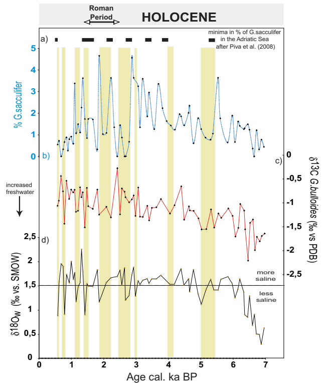
Fig. 5. Comparison of the surface dwelling foraminifera Globigerinoides sacculifer abundance and hydrological changes in core MD90–917 vs. age (cal. ka BP). (a) G. sacculifer minima events recorded in the Adriatic Sea (Piva et al., 2008). (b) Percentage of G. sacculifer in core MD90–917. (c) \delta^{13}\text{C} of the planktonic foraminifera G. bulloides . (d) Sea water \delta^{18}\text{O} record ( \delta^{18}\text{O}_w ). Yellow bars indicate \delta^{18}\text{O}_w /salinity and G. bulloides \delta^{13}\text{C} minima.
