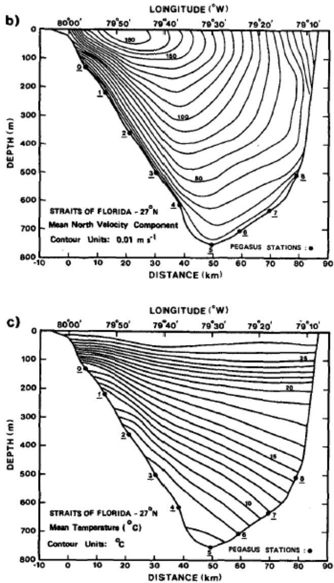
Figure 7: Time average velocity (upper) and temperature field in the modern Florida Current near Miami (Leaman et al. 1987). The bottom velocity is almost everywhere 10cm/s and note the complex structure of the temperature field, with significant shifts in the inter-isotherm distances on the east. They also display the standard deviations of these fields. Little seems understood of how the temporal variability affects the paleotemperature proxies.
