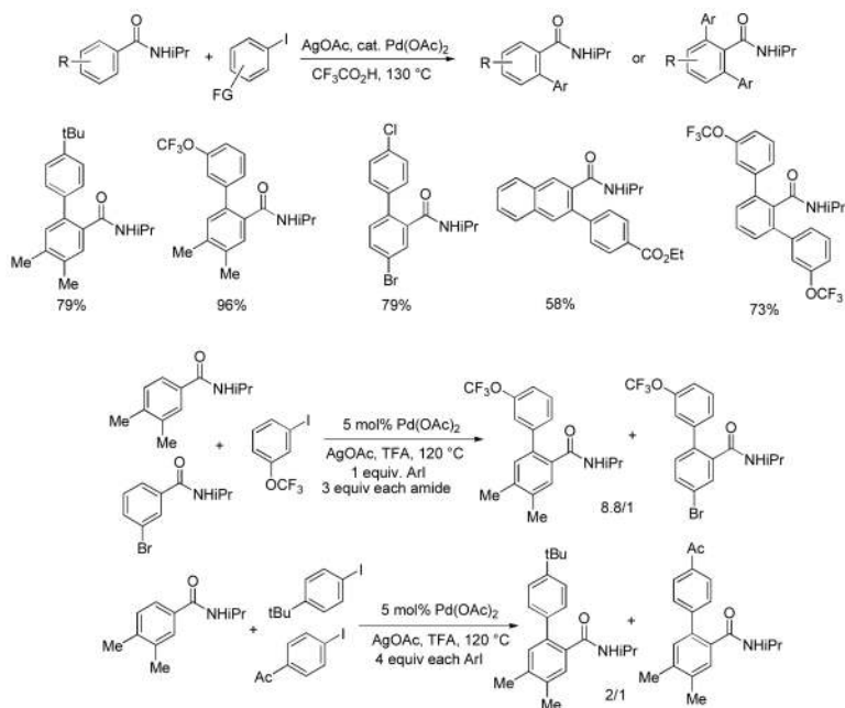
Scheme 3. Benzamide Arylation
