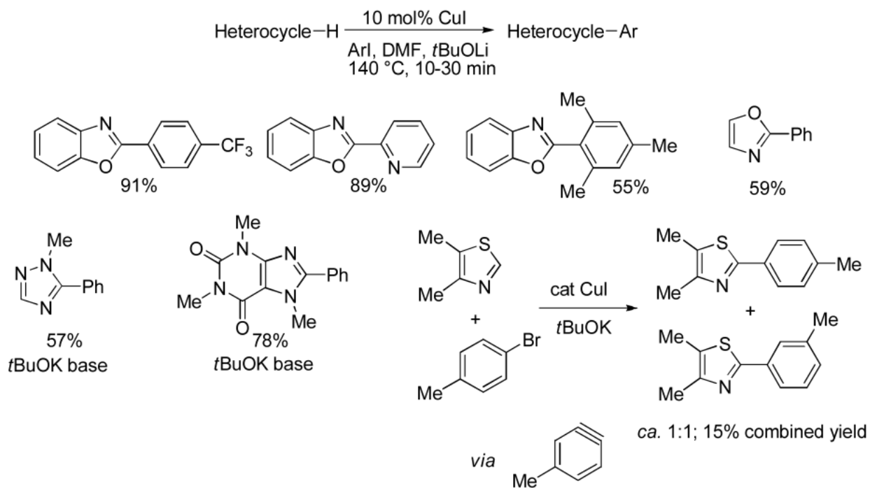
Scheme 12. Copper-Catalyzed Arylation of Acidic Heterocycles
