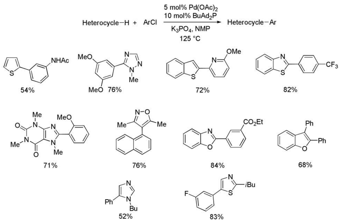
Scheme 11. Heterocycle Arylation by Aryl Chlorides
