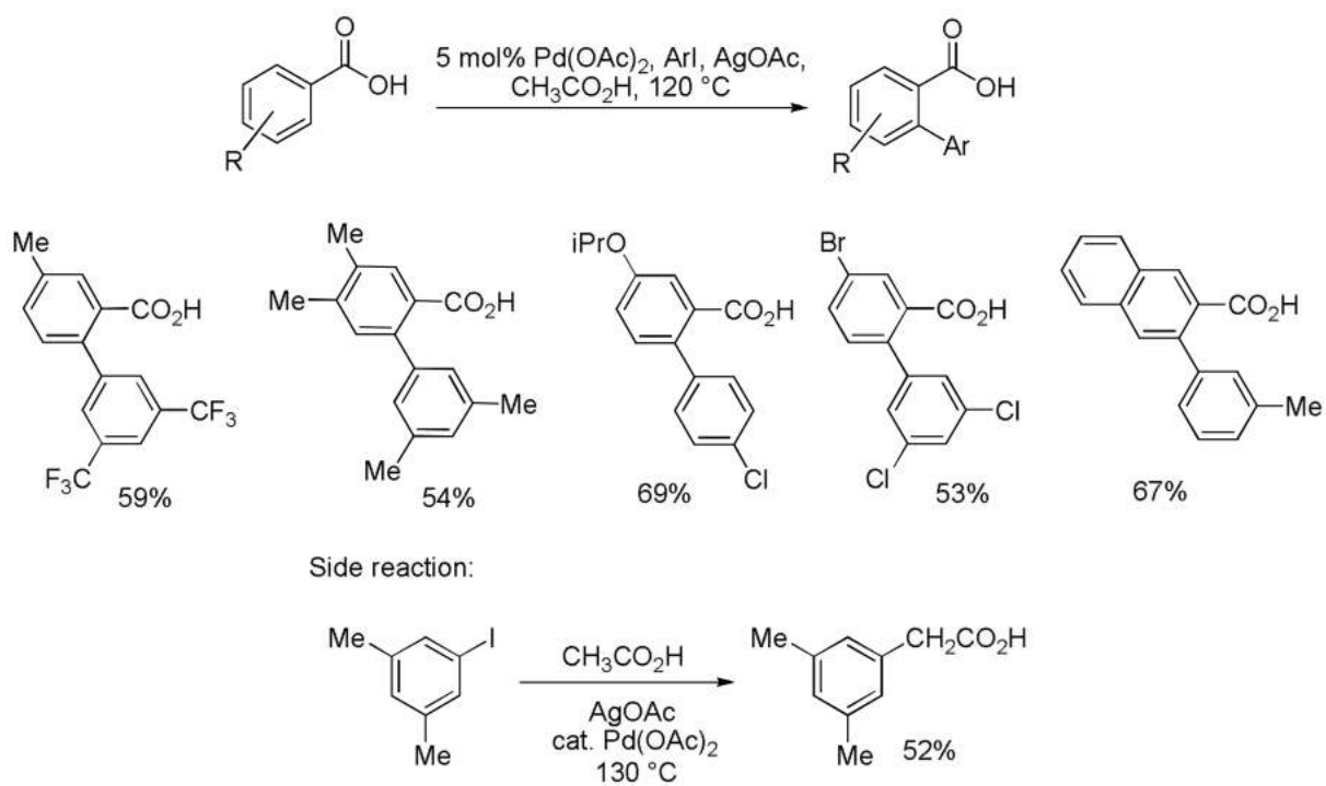
Scheme 4. Benzoic Acid Arylation
