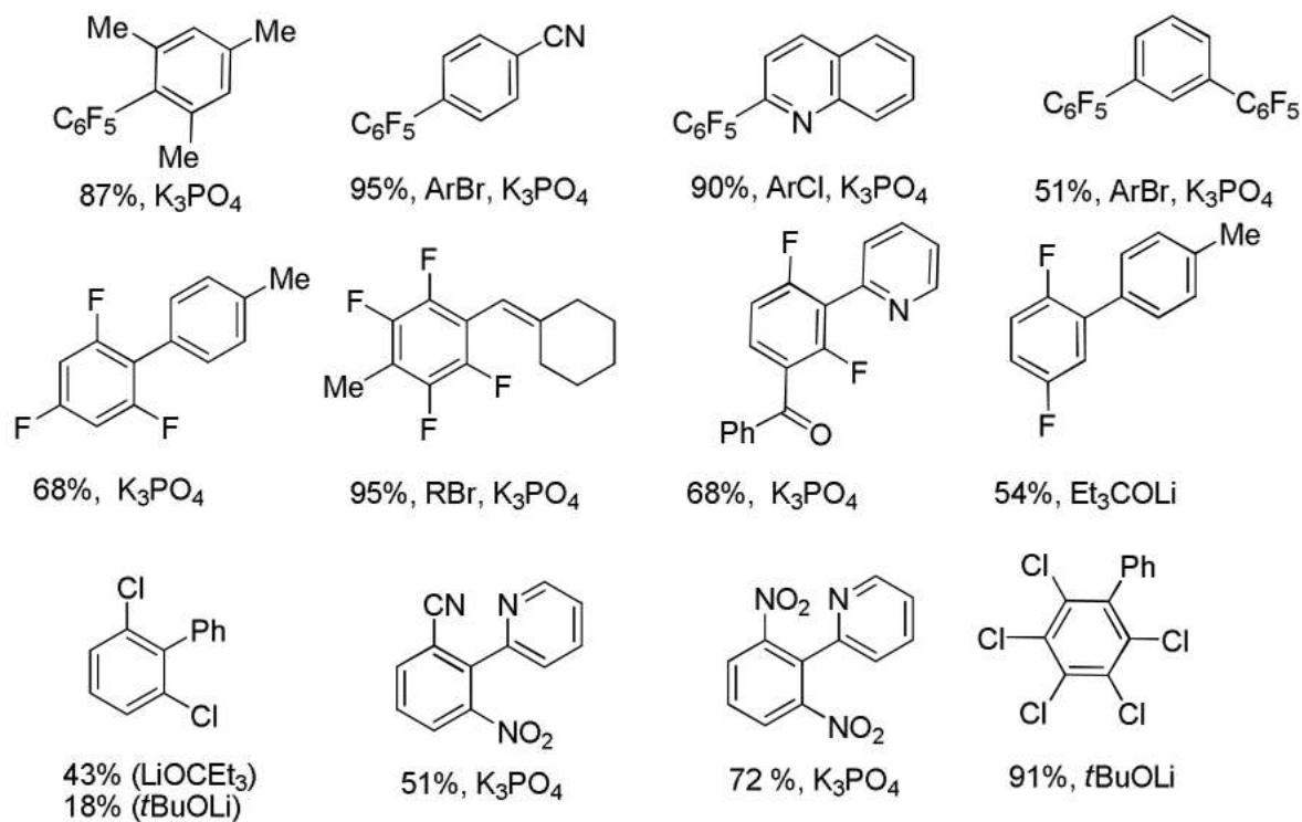
Scheme 15. Electron-Deficient Benzene Arylation
