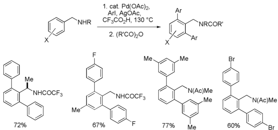
Scheme 6. Benzylamine Arylation
