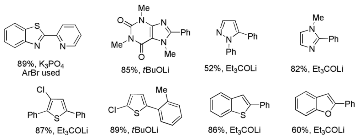
Scheme 13. Electron-Rich Heterocycle Arylation
