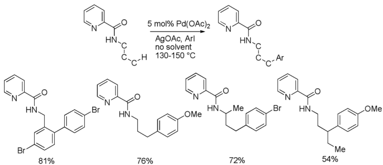
Scheme 9. Amine Derivative Arylation
