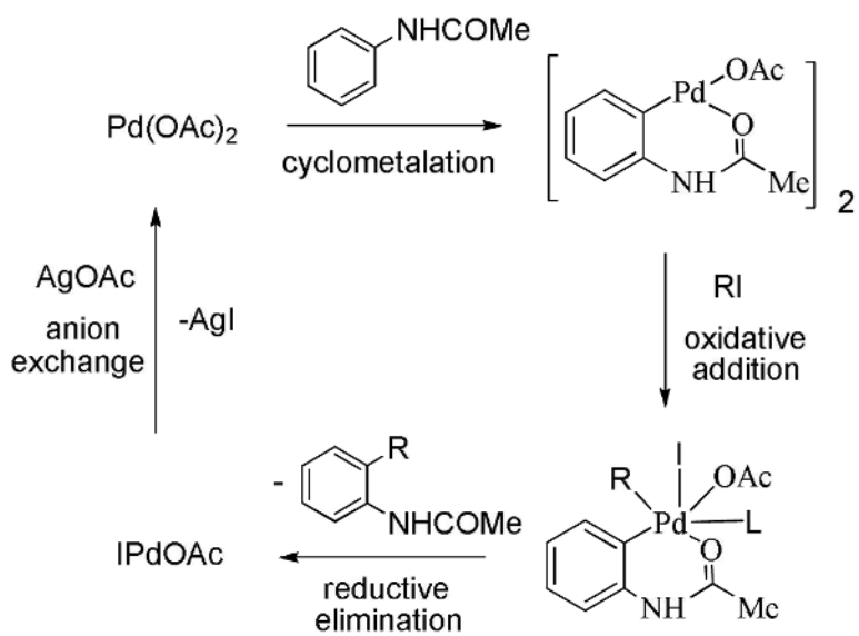
Scheme 1. Catalytic Cycle
