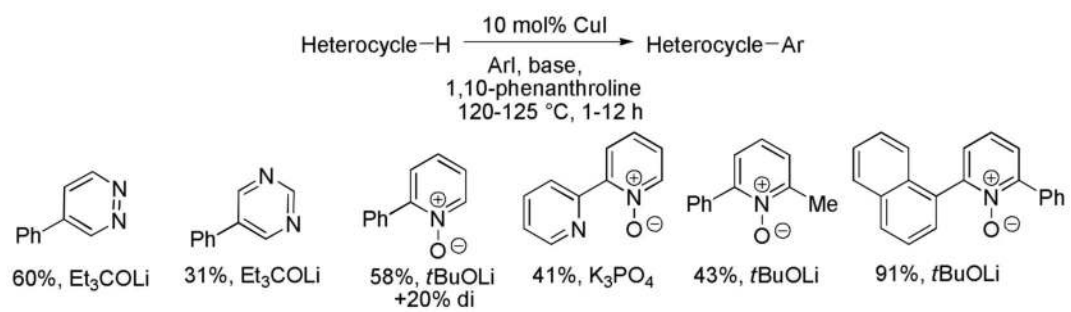
Scheme 14. Electron-Deficient Heterocycle Arylation
