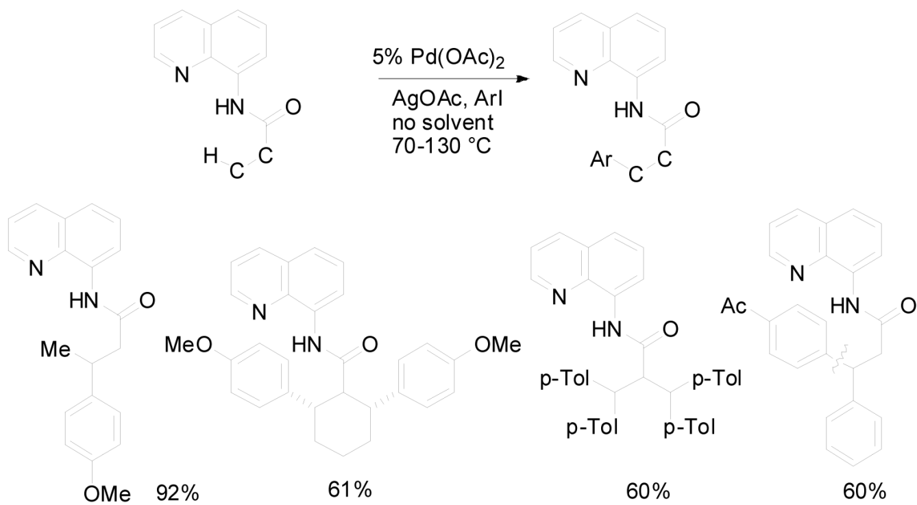
Scheme 8. Carboxylic Acid Derivative Arylation
