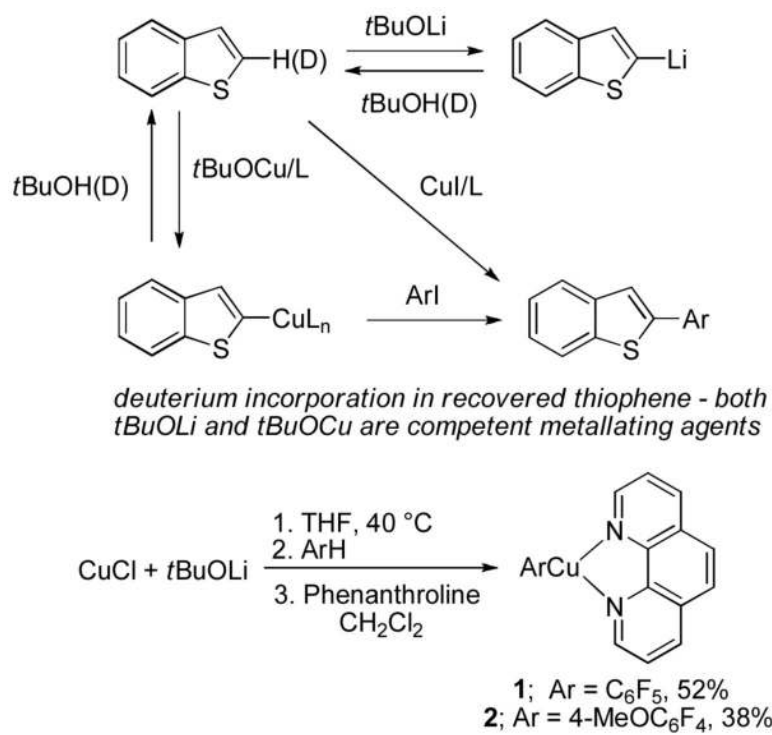
Scheme 16. Mechanistic Considerations
