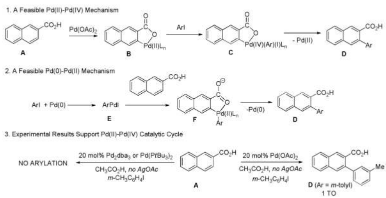
Scheme 5. Mechanistic Considerations
