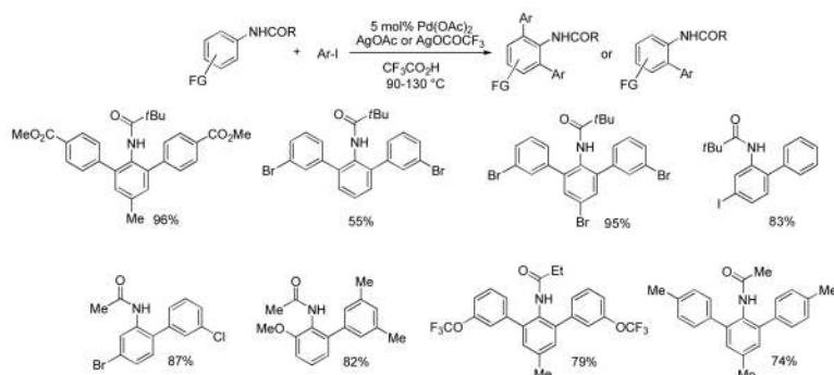
Scheme 2. Anilide Arylation
