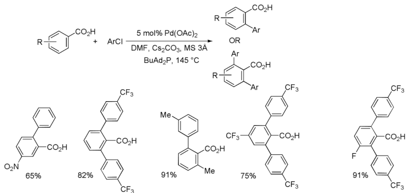
Scheme 10. Benzoic Acid Arylation by Aryl Chlorides
