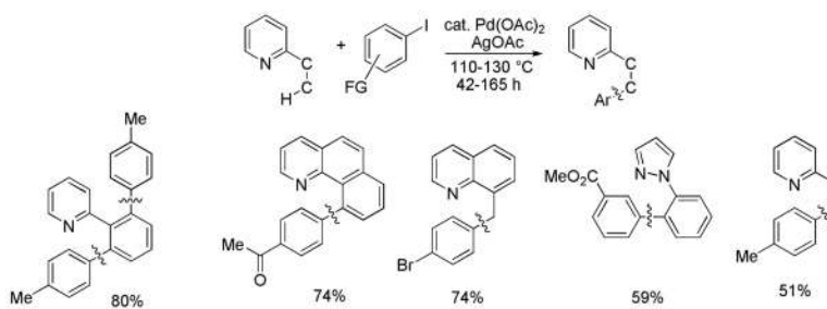
Scheme 7. Pyridine and Pyrazole Derivative Arylation
