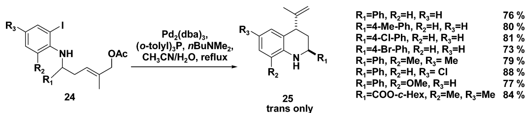
Scheme 8
