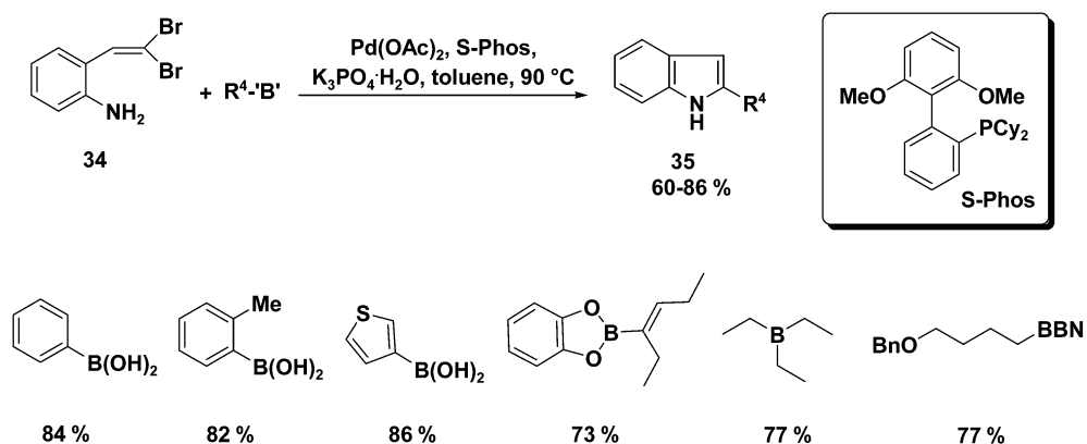
Scheme 12
