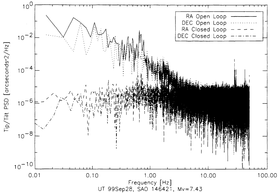
Figure 2. The open and closed loop tip/tilt PSD while observing SAO 146421
