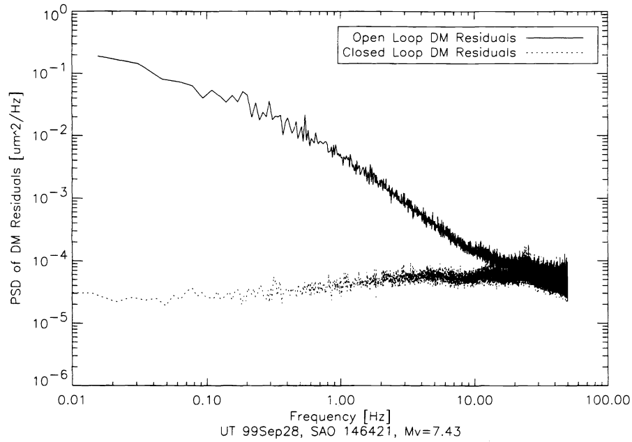
Figure 4. The power spectral density (PSD) of the open and closed loop DM residuals. The open loop DM residuals are a measure of the atmospheric phase errors. The PSDs were calculated for each DM actuator and then averaged. The servo bandwidth is about 15 Hz.
