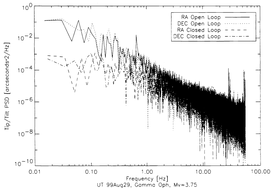
Figure 1. The open and closed loop tip/tilt PSD while observing Gamma Oph
