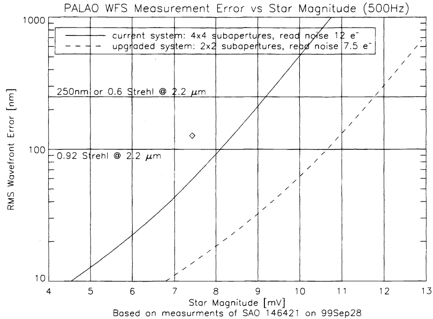
Figure 5. The WFS measurement noise (using Eq. 9) as a function of guide star magnitude. The solid line is the theoretical curve for the current system and the dashed line (which assumes an r_0 of 15 cm) is that for a planned upgrade to a new wavefront sensor. 14 The data point at mV=7.43 and \sigma_{WFS} = 127 nm is the measured value.
