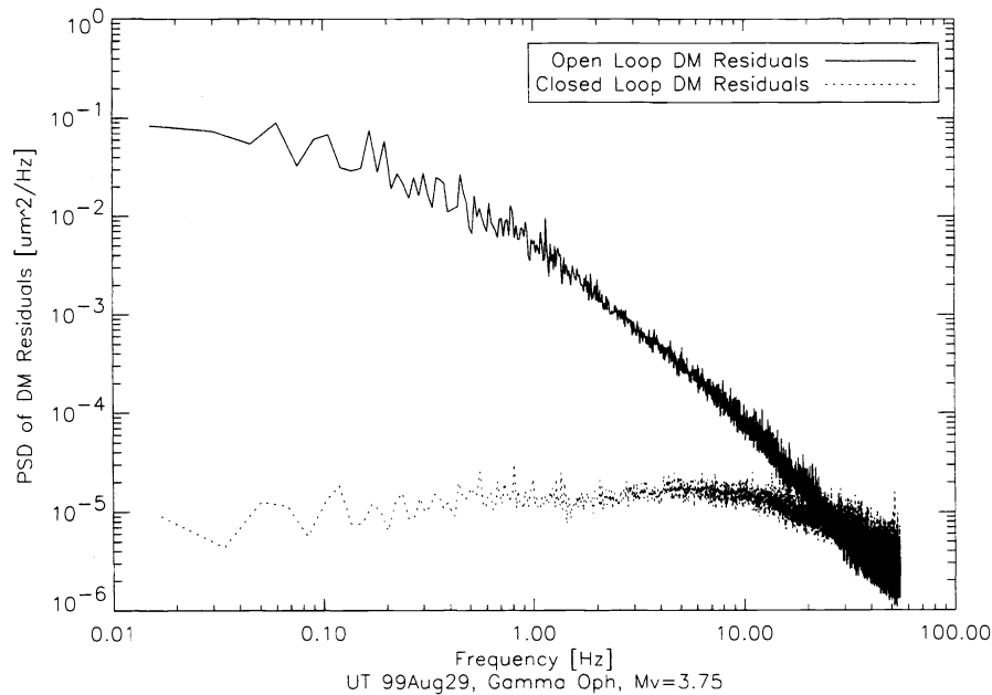
Figure 3. The power spectral density (PSD) of the open and closed loop DM residuals. The open loop DM residuals are a measure of the atmospheric phase errors. The PSDs were calculated for each DM actuator and then averaged. The servo bandwidth is about 15 Hz.
