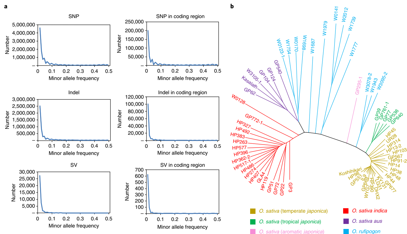
Fig. 1 | Whole-genome variants from 66 representative rice genomes. a , Allele frequency spectra for the indicated kinds of genetic variants. For each variant, we identified the minor allele across the 66 accessions and calculated the frequency of this allele. b , Neighbor-joining tree of the 66 accessions using whole-genome data. The accessions within different groups are indicated by different colors.
