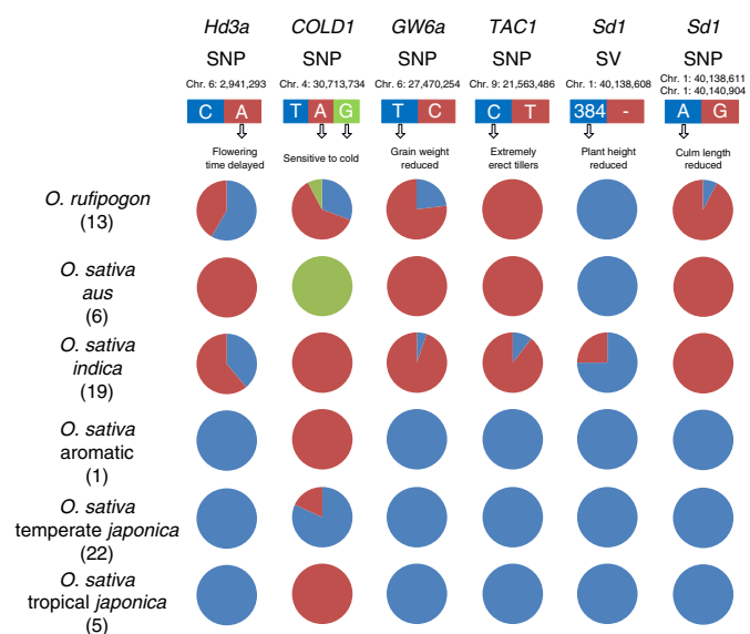
Fig. 2 | Allele frequencies of the causal polymorphisms for the Hd3a , COLD1 , GW6a , TAC1 and Sd1 genes in different O. sativa and O. rufipogon groups. The type of reference allele is indicated in blue, and the alternative one is indicated in red or green.
