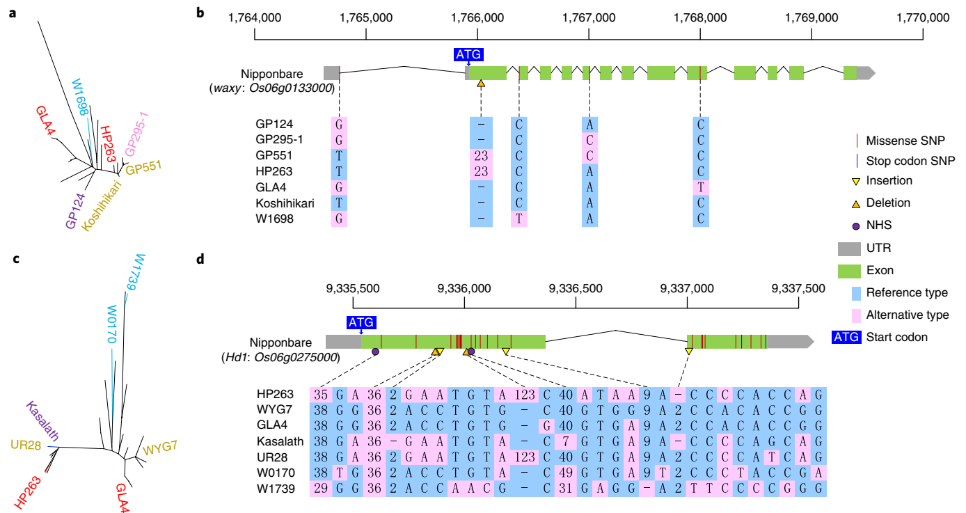
Fig. 3 | Multiple alleles in waxy and Hd1 . a , Neighbor-joining tree of 66 accessions using genetic variants in waxy . Seven diverse accessions representing different haplotypes were selected from the tree and are color-coded according to rice group. b , Allelic information of sequence variants in waxy for the seven accessions. c , Neighbor-joining tree using genetic variants in Hd1 . d , Allelic information of sequence variants in Hd1 for the seven accessions selected in c .
