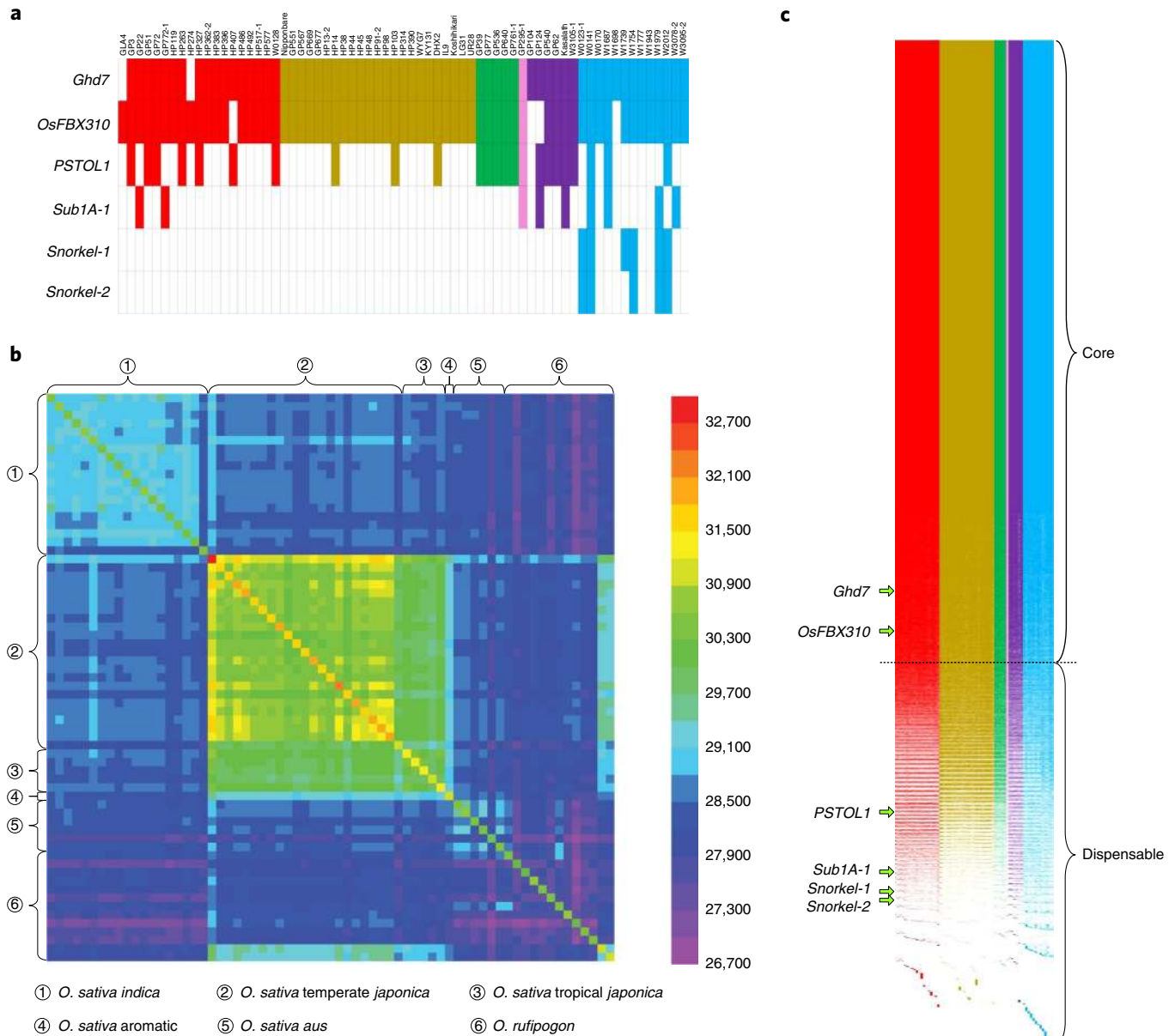
Fig. 5 | PAV of coding genes in the rice genome. a , PAV of six functionally characterized genes in the 67 genomes. The accessions within different groups are color-coded as in Fig. 1b. The absence of a gene in the genome is indicated by a blank box. b , A 67 × 67 matrix comparing the coding genes of the accessions by pairs. For each rice accession, we searched for the genes it shared with each of the 67 accessions. The color index corresponds to the number of shared coding genes. c , Presence and absence information of 42,580 genes in the 67 rice accessions. The order of the 67 accessions (from “GLA4” on the left to “W3095-2” on the right) is the same as in a . The core genome set and the dispensable genome set refer to coding genes present in ≥90% of rice accessions and genes present in <90% of accessions, respectively. Presence is color-coded as in a , and the absence of a gene is indicated by white.
