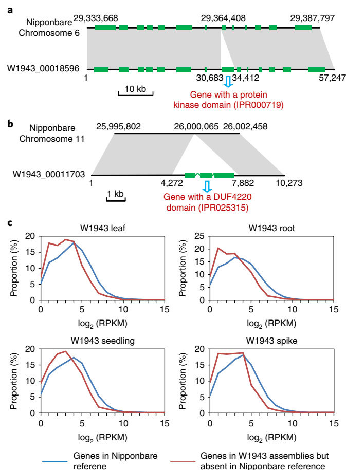
Fig. 4 | Newly identified genes in O. rufipogon W1943. a , Detection of an expressed gene on chromosome 6 of the W1943 genome assembly in a 3.7-kb insertion. The black lines and green boxes indicate genome sequences and gene-coding regions, respectively. Domain information from InterPro scans is indicated. b , Detection of an expressed gene on chromosome 11 of the W1943 assembly in an insertion of 3.6 kb. c , Comparison of the expression levels of genes annotated in the Nipponbare reference and the newly identified genes in the W1943 genome in four tissues of W1943.
