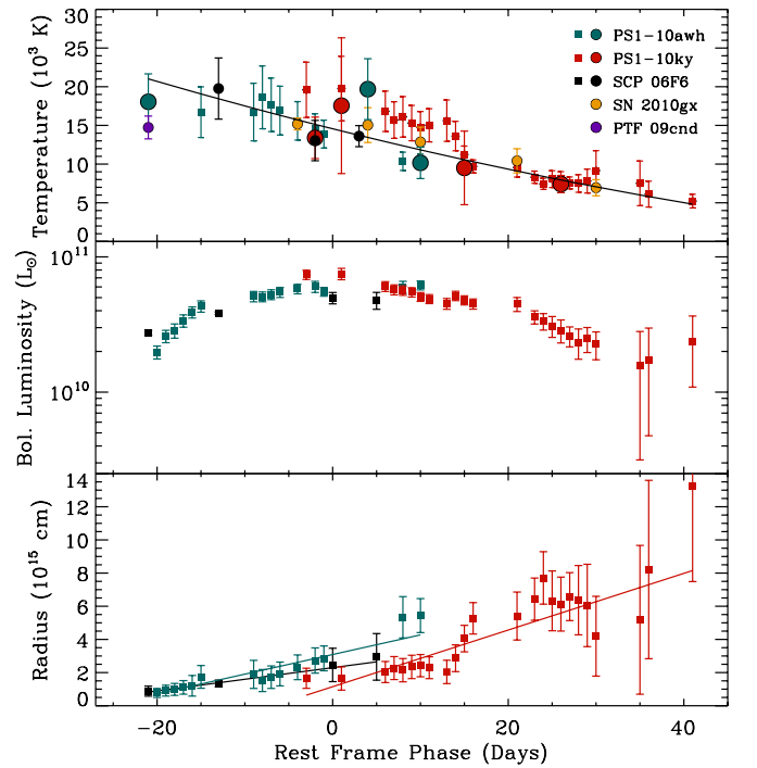
Figure 8. Top panel: temperature as a function of rest-frame time. Squares denote measurements from photometry, while circles are spectroscopic measurements. The quadratic fit to the PS1-10ky and PS1-10awh data is marked as a black solid line. Measurements for PS1-10awh are in blue, PS1-10ky in red, SCP 06F6 in black, SN 2010gx in gold, and PTF09cn in violet. Middle panel: bolometric luminosity as a function of time. These are determined by summing up flux in the measured photometric bands and extrapolating a blackbody tail to the red; emission blueward of 2100 Å (rest frame) for PS1-10ky/PS1-10awh and 3150 Å for SCP 06F6 is not accounted for, implying that these are lower limits. Bottom panel: radius as a function of time, assuming the bolometric luminosities from the middle panel and the temperatures from the top panel. Linear fits are marked by solid lines. In the middle and bottom panels, colors denote PS1-10ky, PS1-10awh, and SCP 06F6 as in the top panel.
