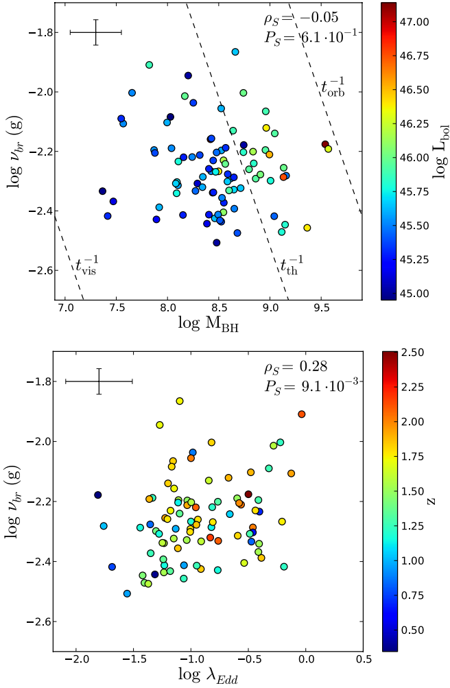
Fig. 14. Optical break frequency ( g_{P1} band PSD_MBH sample) versus M_{\text{BH}} , color coded with L_{\text{bol}} (top) and \lambda_{\text{Edd}} , color coded with redshift (bottom). The black error bars are the average values. There is no significant evidence for a correlation with these AGN parameters. The dashed lines in the top panel correspond to the expected scaling of the orbital, thermal and viscous timescales at 10R_S , see text for details.
