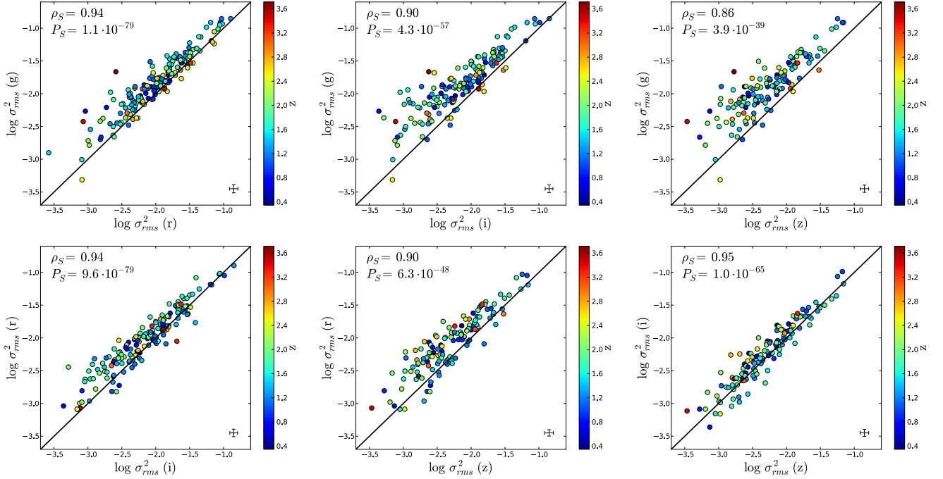
Fig. 3. Comparing the excess variance measured on timescales of years in the different PS1 bands. The data of all objects from the total sample with variability information in both considered bands are shown. The Spearman correlation coefficient and the respective p -value are reported in each subpanel. The redshift is given as a color bar. The black line corresponds to the one-to-one relation. The black error bars are the average values.
