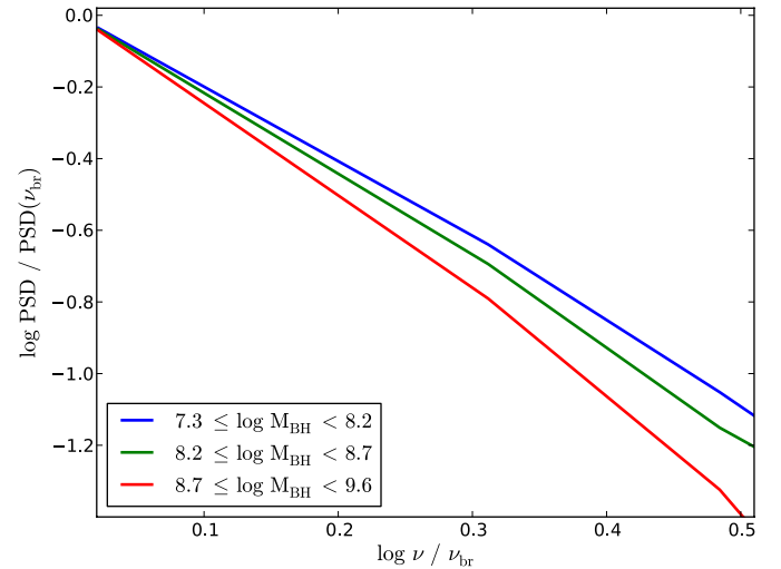
Fig. 17. High-frequency PSD ( g_{P1} band PSD_MBH sample) for three bins of black hole mass. We show the sample median for each M_{BH} bin after normalizing the PSD to the values at \nu_{br} in order to transform the PSD of each AGN to the same unit scale.
