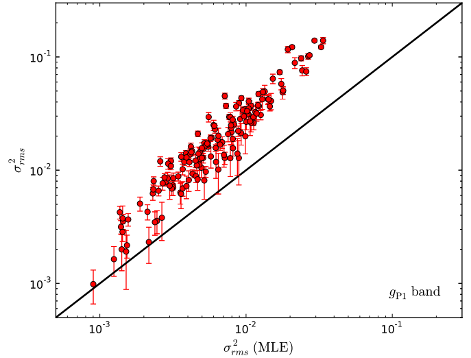
Fig. 13. Comparison of the integral of the maximum-likelihood estimate of the PSD, \sigma_{\text{rms}}^2(\text{MLE}) , with the excess variance \sigma_{\text{rms}}^2 calculated after Eq. (1). The data for the g_{\text{P1}} band PSD sample are shown. The black line corresponds to the one-to-one relation.
