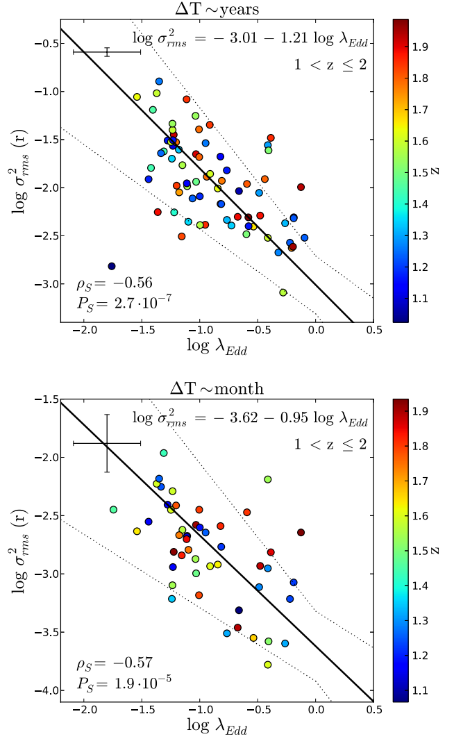
Fig. 8. Excess variance ( r_{P1} band) measured on timescales of years ( top ) and months ( bottom ) versus \lambda_{\text{Edd}} for the 1z2_MBH sample. The best-fit power law and other symbols are displayed as in Fig. 5.
