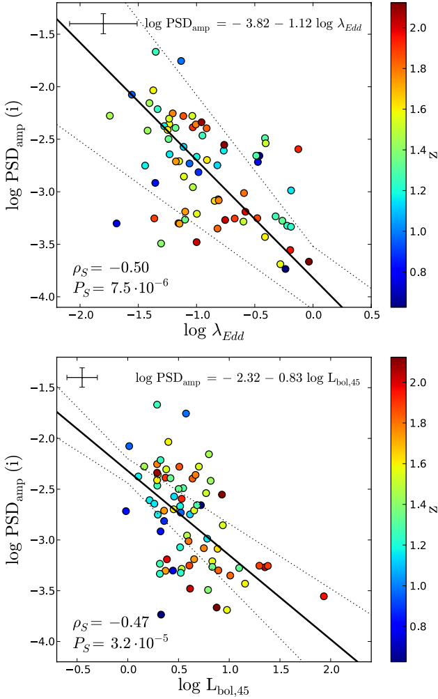
Fig. 15. PSD amplitude ( i_{P1} band PSD_MBH sample) versus \lambda_{Edd} (top) and L_{bol} (bottom). The redshift is given as a color bar. The best-fit power law and other symbols are displayed as in Fig. 5.
