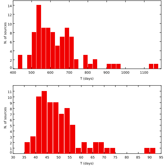
Fig. 1. Top panel: histogram of the rest-frame observation length of the total light curve for the year timescale MBH sample ( g_{P1} band). Bottom panel: histogram of the rest-frame observation length (average value of the light-curve segments) for the month timescale MBH sample ( g_{P1} band).
