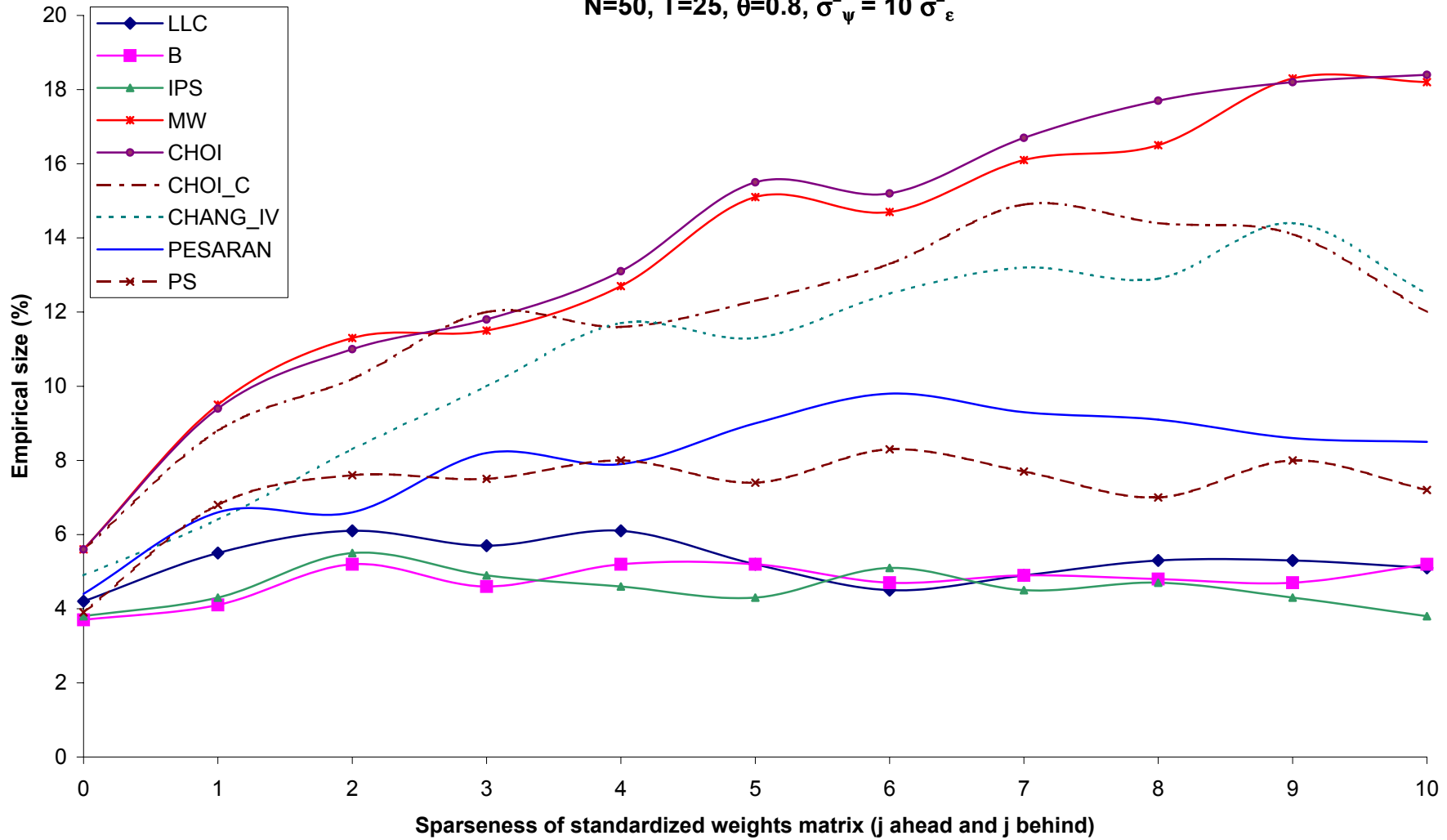
Fig. 5 - Spatial Error Component process (SEC3)
