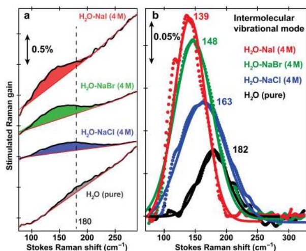
Fig. 2 Inter-molecular H-bond stretching mode in H 2 O and aqueous salt solutions. Ground-state FSRS spectra of pure water (black) and aqueous solutions with 4 M halide salts: NaCl (blue), NaBr (green), and NaI (red) raw data are shown with the baselines in (a), and after pure water peak subtraction (except for water itself) and baseline removal in (b), respectively. The 580 nm Raman pump power is set at 4 mW (see the ESI † ). Careful steps were taken to reduce scattering in the low-frequency region (<350 cm -1 , see Experimental). The stimulated Raman gain magnitude is indicated by the double-headed vertical line.
