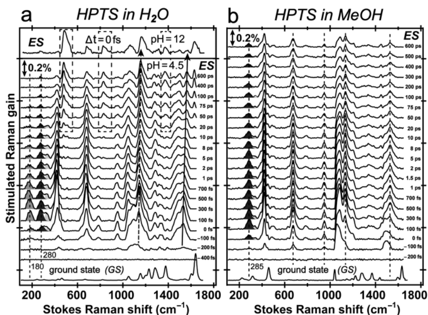
Fig. 3 Time-resolved excited-state FSRS spectra between ca. 100–1700 \text{cm}^{-1} of 1.5 mM HPTS in water and methanol following 400 nm photoexcitation up to 600 ps. (a) HPTS in \text{H}_2\text{O} at pH=4.5. The S_1 FSRS data ( \Delta t=0 fs) at pH=12 is shown above. Dashed boxes highlight the emerging modes at later time of the chemical reaction. The blueshift of the \sim 1140 and 1530 \text{cm}^{-1} modes is denoted by dashed and solid curved arrow, respectively. (b) HPTS in methanol. The dashed lines indicate largely unchanged Raman peak position in S_1 as molecular structure responds to photoexcitation. The solvent-subtracted ground-state spectra are plotted at the bottom for comparison with the ground-state-subtracted excited-state spectra as a function of time delay (noted on the right to each trace) between the femtosecond actinic pump and Raman probe pulses.
