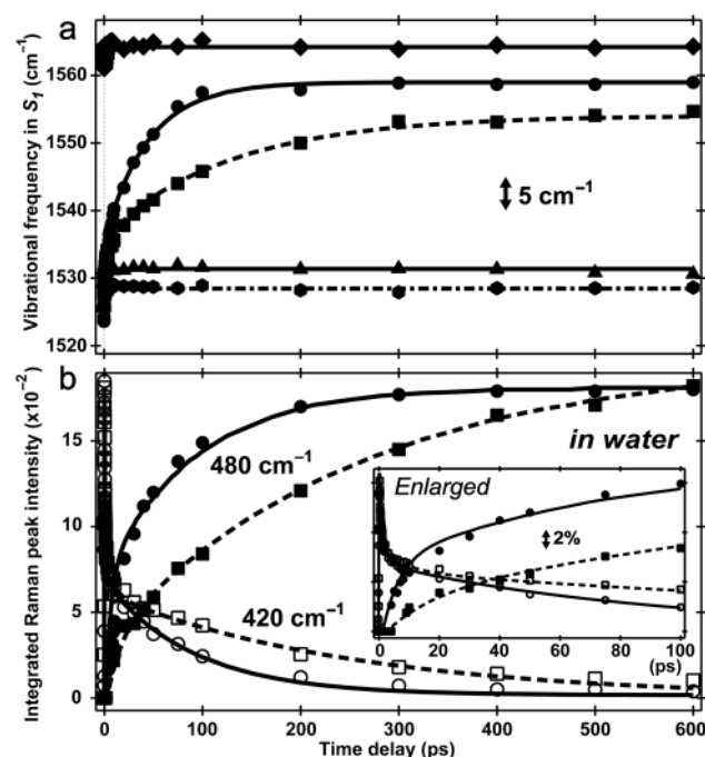
Fig. 4 Excited-state vibrational frequency and intensity dynamics for marker bands of 1.5 mM HPTS and MPTS in various solvents up to 600 ps. (a) The high-frequency mode frequency shift of HPTS in aqueous basic solution (pH=12, diamond), H 2 O (pH=4.5, circle), D 2 O (pD=4.5, square), methanol (hexagon), and MPTS in H 2 O (triangle). The double-exponential fits are shown for HPTS in H 2 O (solid) and D 2 O (dashed) with pronounced mode blueshift. Straight lines indicate unchanged frequencies at \sim 1530 cm -1 for HPTS in methanol (dash-dotted) and MPTS in H 2 O (solid), and at \sim 1564 cm -1 for HPTS in basic solution (solid line). (b) Intensity dynamics of the 420/480 cm -1 S 1 Raman modes for HPTS in H 2 O (hollow circle/solid circle) and D 2 O (hollow square/solid square). Kinetic isotope effect of \sim 3 is apparent (see ESIT + ). The enlarged plot within 100 ps is shown in the insert with the stimulated Raman gain magnitude depicted by the double-angled vertical line.
