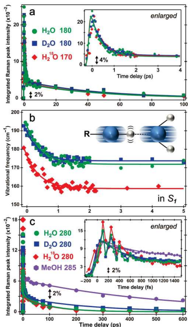
Fig. 5 Excited-state intensity and frequency evolution of \sim 180 and 280 \text{cm}^{-1} modes of 1.5 mM HPTS in various solvents following fs 400 nm photoexcitation. Time-resolved (a) integrated intensity dynamics and (b) frequency shift of the 180 \text{cm}^{-1} S_1 mode in \text{H}_2\text{O} (pH=4.5, green circle) and \text{D}_2\text{O} (pD=4.5, blue square), and 170 \text{cm}^{-1} mode in \text{H}_2^{18}\text{O} (pH=4.5, red diamond) are overlaid with multi-exponential fits (solid traces), respectively. The enlarged plot up to 4 ps is shown in (a) insert. The intermolecular O–H...O stretching motion is illustrated in (b) insert. The oxygen/hydrogen atom is shown as blue/white sphere, respectively, with the shadows and wiggles mapping their vibrational trajectories. (c) Intensity dynamics of the 280 \text{cm}^{-1} mode in \text{H}_2\text{O} (green circle), \text{D}_2\text{O} (blue square) and \text{H}_2^{18}\text{O} (red diamond), and 285 \text{cm}^{-1} mode in MeOH (magenta hexagon) up to 600 ps. The enlarged plot with coherent spectral oscillations (except for MeOH) superimposed on the \sim 280 \text{cm}^{-1} mode integrated intensity decay up to 1.5 ps is shown in the insert.
