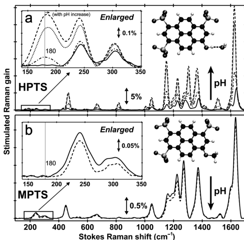
Fig. 1 Ground-state FSRS of 40 mM HPTS and 20 mM MPTS in \text{H}_2\text{O} . (a) HPTS in \text{H}_2\text{O} at pH=4.5 (solid), 7 (dash-dotted), 9 (dotted), and 12 (dashed line) from ~100–1700 \text{cm}^{-1} . The enlarged low-frequency region between 140–350 \text{cm}^{-1} is shown in the insert (left). (b) MPTS in \text{H}_2\text{O} at pH=4.5 (solid) and 12 (dashed line). The enlarged low-frequency region is shown. Molecular structures of HPTS (H-bonded to one nearby water molecule) and MPTS are depicted in the insert (right). Carbon, oxygen, and hydrogen atoms are depicted in black, dark gray, and white spheres, respectively. The Raman gain magnitude is indicated by the double-headed line. The largely featureless aqueous solvent blank spectrum has been subtracted. Notably, we only use this high sample concentration to enhance ground-state vibrational peaks particularly in the low-frequency region.
