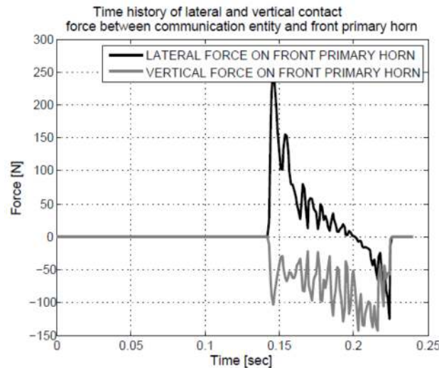
Figure 14 - Time histories of lateral contact load (black solid line) and vertical contact load (grey solid line) over crash test on simple pre-tensioned CW
