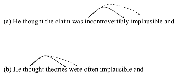
Figure 1: (a) Mis-location leading to an unintended re-fixation; (b) mis-location following a failed skip leading to an erroneous single fixation. Dotted lines show the intended target and solid lines the actual saccade executed.
