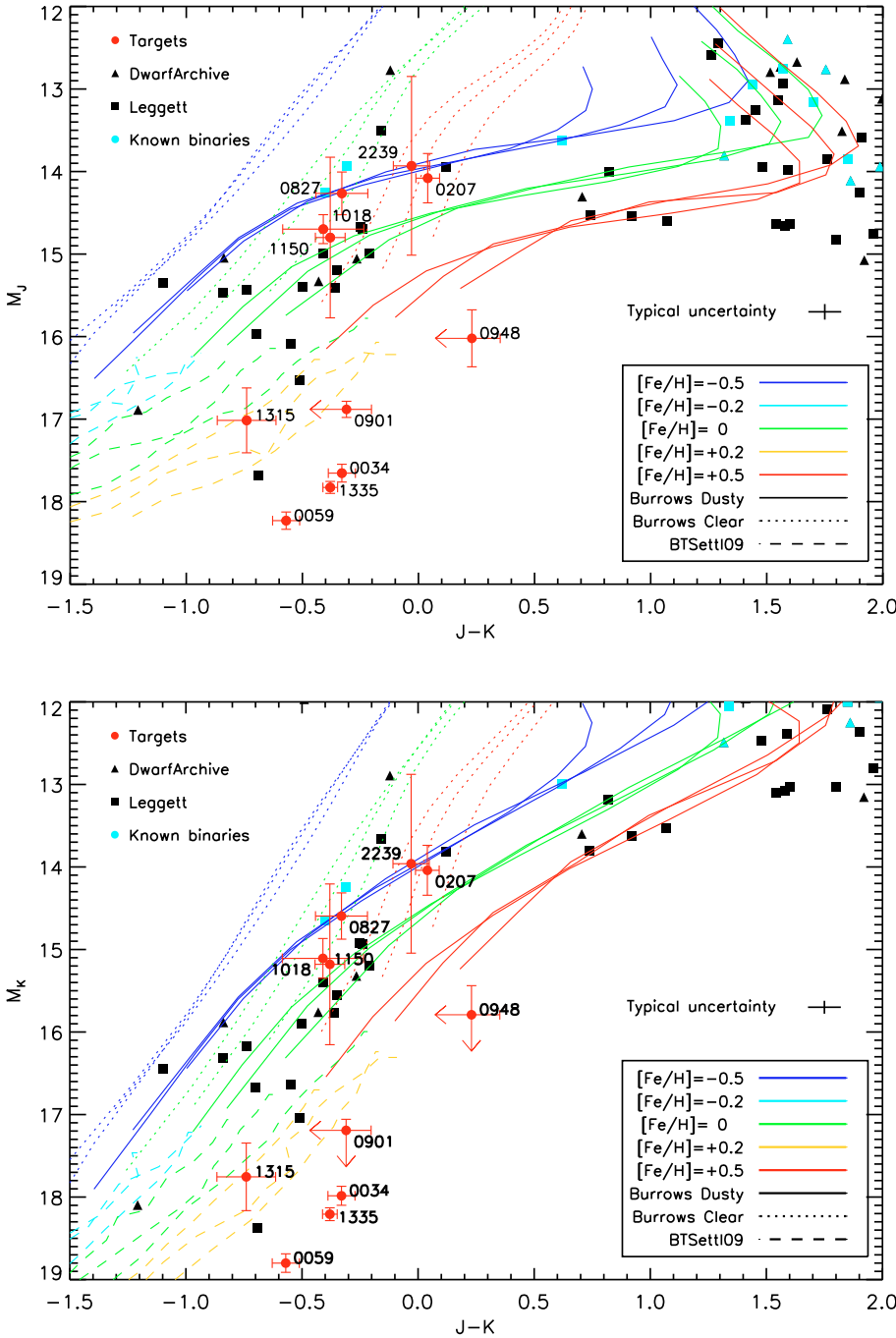
Fig. 3. Same as Fig. 2 but with the color J - K instead of J - H . For each metallicity, the gravity increases from right to left, assuming the values 4.5, 5.0, 5.5 for BSH06 tracks and 4.5, 5.0, 5.25 for BTSettl09.
