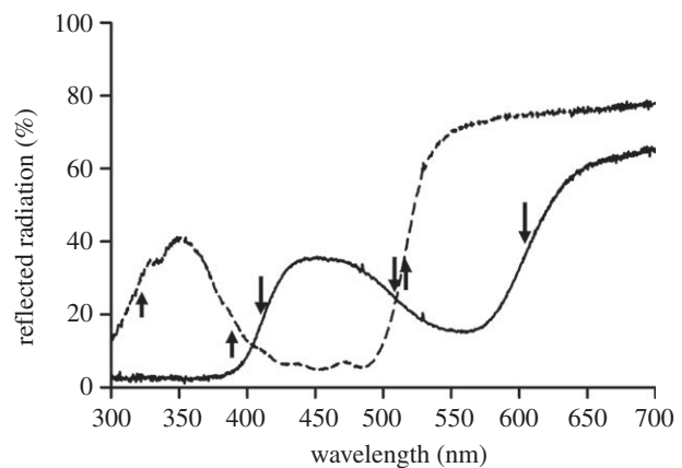
Figure 1. Example floral spectral reflections of two Australian native flowers (endemic): Hibbertia scandens (dashed lines, human yellow) and Pandorea jasminoides (solid line, human pink). The arrows show the slope midpoints [25].
