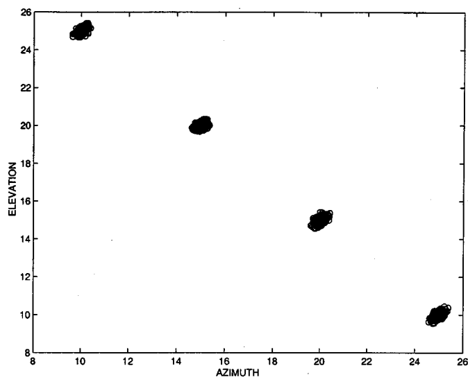
Fig. 4. Azimuth-elevation scatter, SNR = 12 dB.
