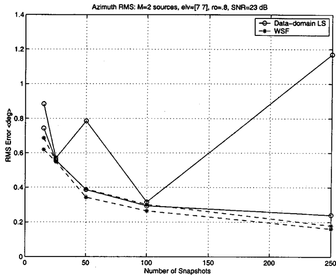
Fig. 10. Azimuth RMSE: Two 0.8-correlated sources, (-10^\circ, 7^\circ) , (-5^\circ, 7^\circ) , SNR = 23 dB.
