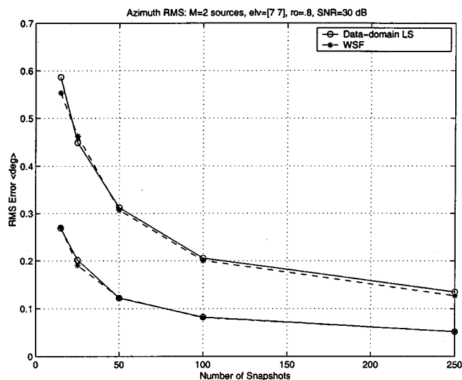
Fig. 8. Azimuth RMSE: Two 0.8-correlated sources, (-10^\circ, 7^\circ) , (-5^\circ, 7^\circ) , SNR = 30 dB.
