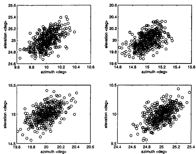
Fig. 5. Azimuth-elevation scatter zoom-in, SNR = 12 dB.
