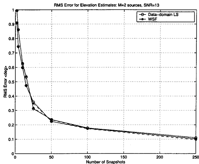
Fig. 7. Elevation RMSE: Two uncorrelated sources, (-10^\circ, 10^\circ) , (-5^\circ, 7^\circ) , SNR = 13 dB.
