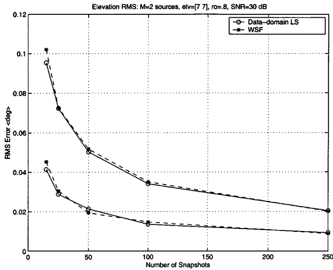
Fig. 9. Elevation RMSE: Two 0.8-correlated sources, (-10^\circ, 7^\circ) , (-5^\circ, 7^\circ) , SNR = 30 dB.
