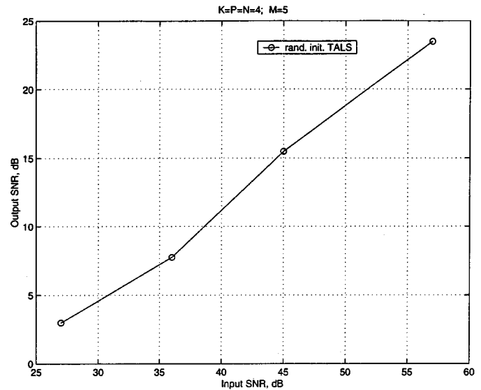
Fig. 12. Average output ( \hat{\mathbf{S}} ) SNR versus input SNR for M = 5 independent complex Gaussian sources, K = P = N = 4 , 1000 Monte Carlo trials.
