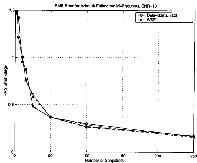
Fig. 6. Azimuth RMSE: Two uncorrelated sources, (-10^\circ, 10^\circ) , (-5^\circ, 7^\circ) , SNR = 13 dB.
