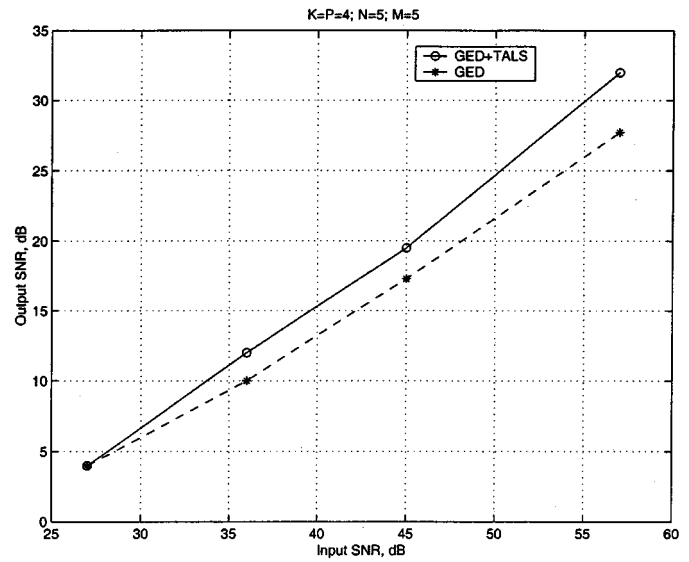
Fig. 11. Average output ( \hat{\mathbf{S}} ) SNR versus input SNR for M = 5 independent complex Gaussian sources, K = P = 4 , N = 5 , 1000 Monte Carlo trials.
