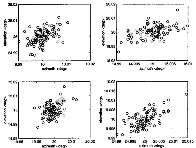
Fig. 3. Azimuth-elevation scatter zoom-in, SNR = 54 dB.
