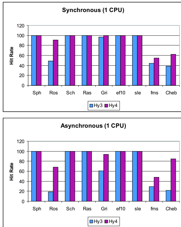
Fig. 11. Hit rate of the Hy3 and Hy4 models (1 CPU).
