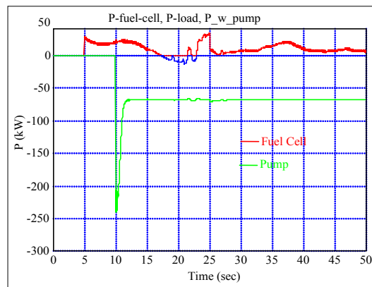
Fig. 11. Output power of fuel cell, water pump
