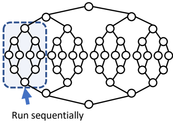
(a) Classic Horizontal Granularity Control (HGC)
