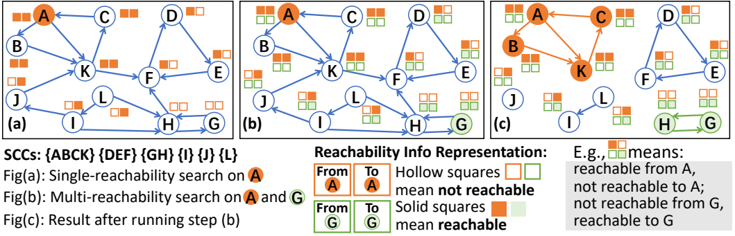
Fig. 2. Example of single- and multi-reachability searches and reachability-based SCC algorithms.
