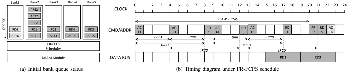
Fig. 5: Command Bus Conflicts for ACT Commands.
