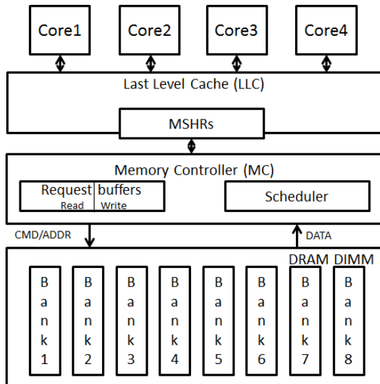
Fig. 1: Modern COTS multicore architecture
