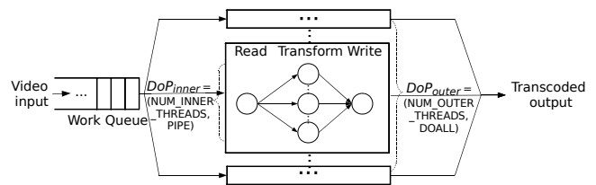
Figure 1. Two-level loop nest in video transcoding: Across videos submitted for transcoding and across frames within each video
